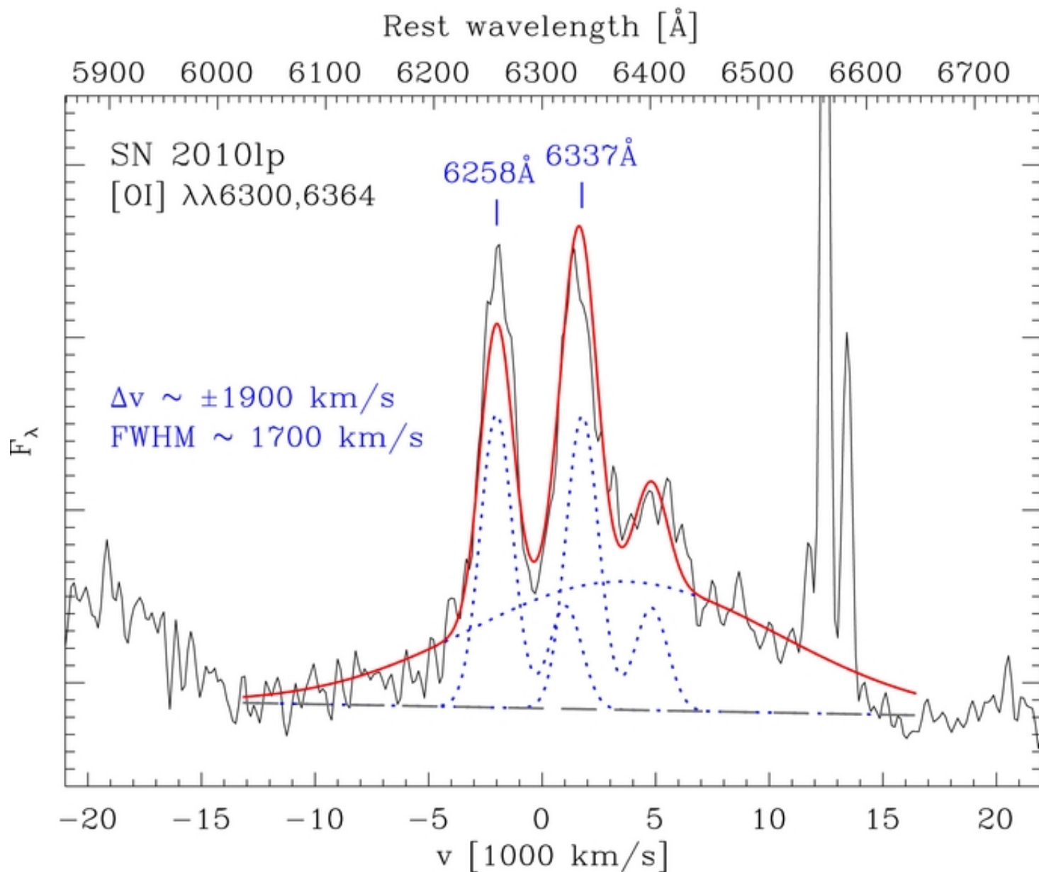
Figure 2. from [O I] 6300, 6364 in the Nebular Spectrum of a Subluminous Type Ia Supernova Taubenberger et al. 2013 ApJL 775 L43 doi:10.1088/2041-8205/775/2/L43 https://dx.doi.org/10.1088/2041-8205/775/2/L43 © 2013. The American Astronomical Society. All rights reserved.
