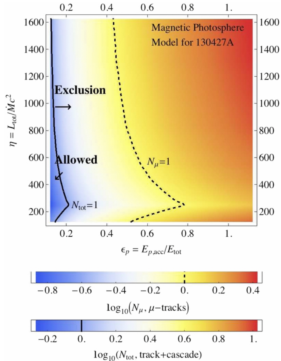
Figure 4. from On the Neutrino Non-detection of GRB 130427A Gao, Kashiyama, & Mészáros 2013 ApJL 772 L4 doi:10.1088/2041-8205/772/1/L4 https://dx.doi.org/10.1088/2041-8205/772/1/L4 © 2013. The American Astronomical Society. All rights reserved.
