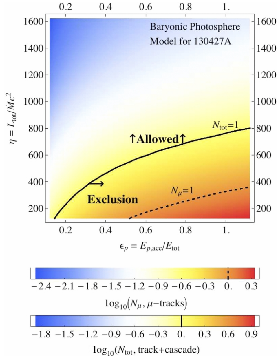
Figure 3. from On the Neutrino Non-detection of GRB 130427A Gao, Kashiyama, & Mészáros 2013 ApJL 772 L4 doi:10.1088/2041-8205/772/1/L4 https://dx.doi.org/10.1088/2041-8205/772/1/L4 © 2013. The American Astronomical Society. All rights reserved.
