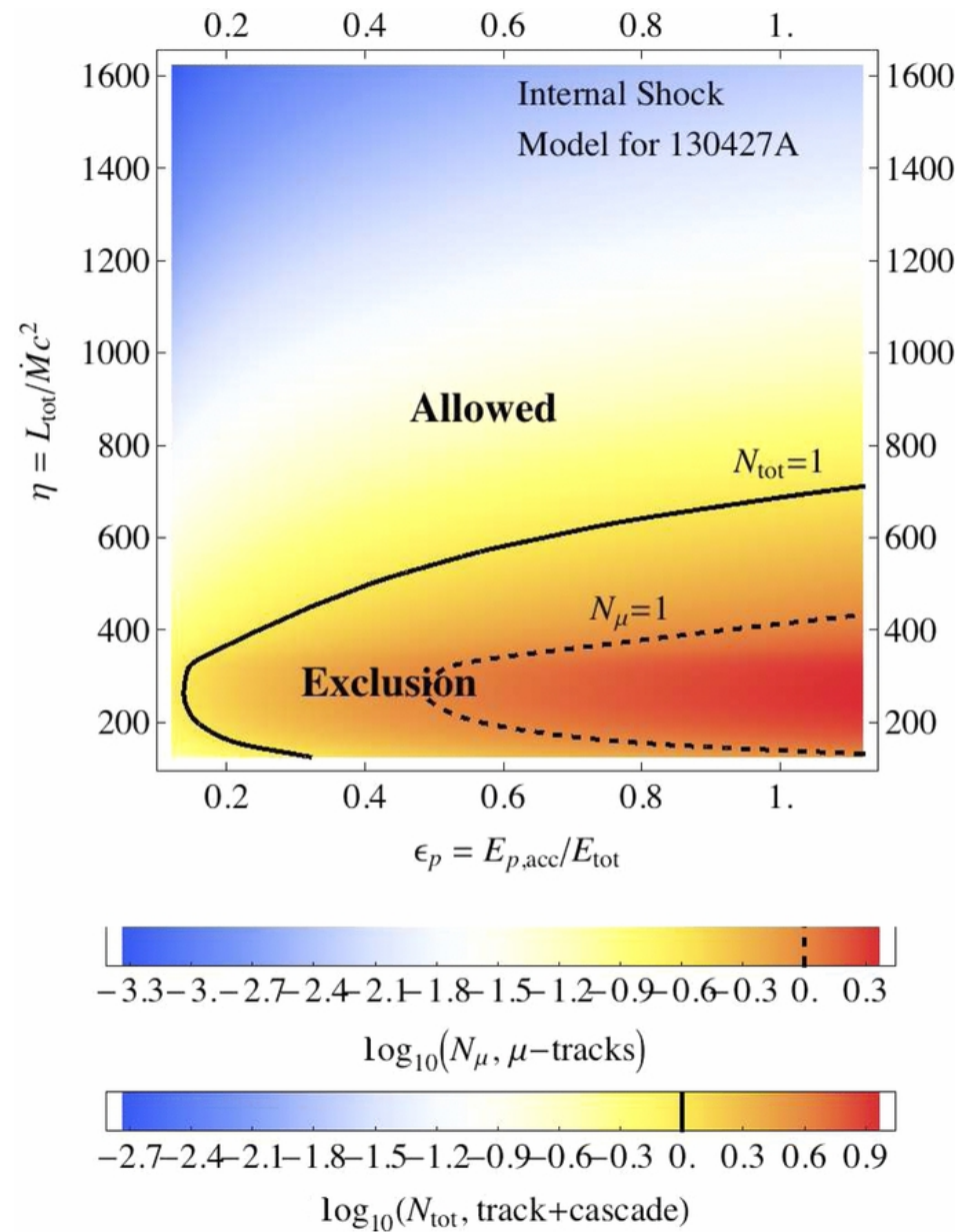
Figure 2. from On the Neutrino Non-detection of GRB 130427A Gao, Kashiyama, & Mészáros 2013 ApJL 772 L4 doi:10.1088/2041-8205/772/1/L4 https://dx.doi.org/10.1088/2041-8205/772/1/L4 © 2013. The American Astronomical Society. All rights reserved.
