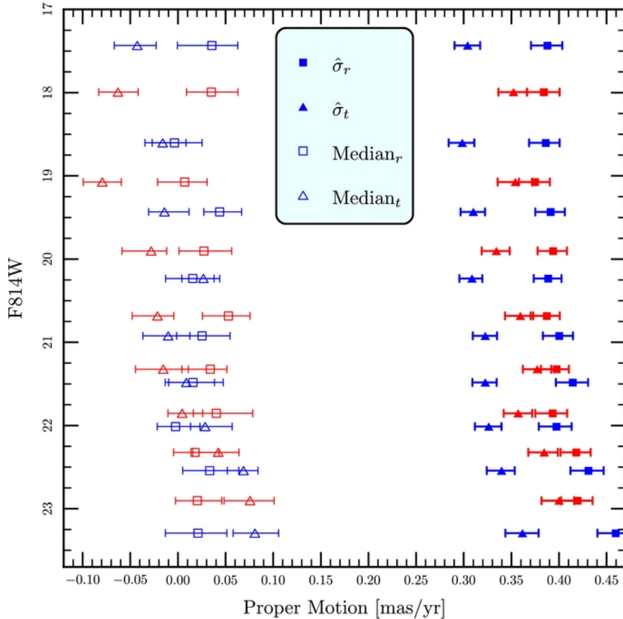
Figure 4. from A Dynamical Signature of Multiple Stellar Populations in 47 Tucanae Richer et al. 2013 ApJL 771 L15 doi:10.1088/2041-8205/771/1/L15 https://dx.doi.org/10.1088/2041-8205/771/1/L15 © 2013. The American Astronomical Society. All rights reserved.
