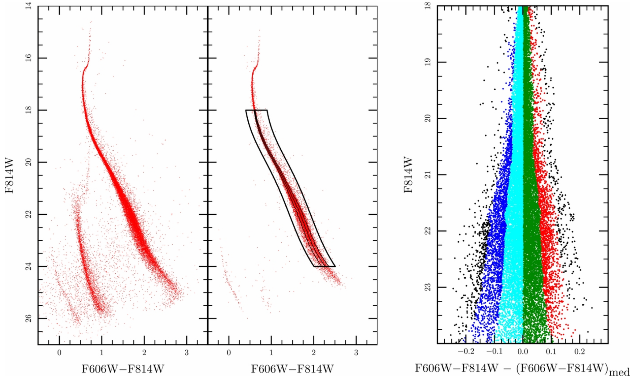
Figure 2. from A Dynamical Signature of Multiple Stellar Populations in 47 Tucanae Richer et al. 2013 ApJL 771 L15 doi:10.1088/2041-8205/771/1/L15 https://dx.doi.org/10.1088/2041-8205/771/1/L15 © 2013. The American Astronomical Society. All rights reserved.
