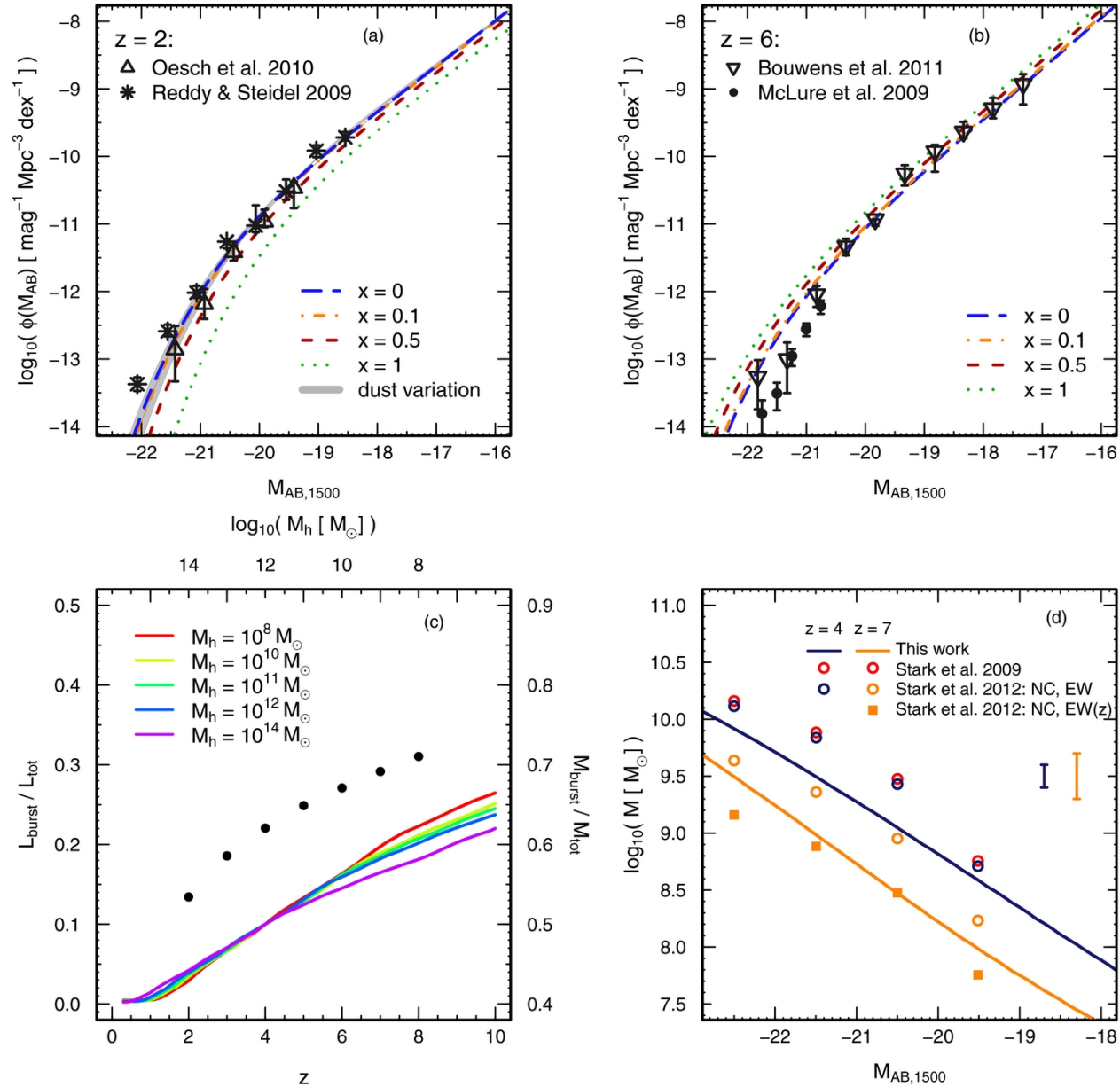
Figure 4. from A Physical Model for the 0 < z < 8 Redshift Evolution of the Galaxy Ultraviolet Luminosity and Stellar Mass Functions Tacchella, Trenti, & Carollo 2013 ApJL 768 L37 doi:10.1088/2041-8205/768/2/L37 https://dx.doi.org/10.1088/2041-8205/768/2/L37 © 2013. The American Astronomical Society. All rights reserved.
