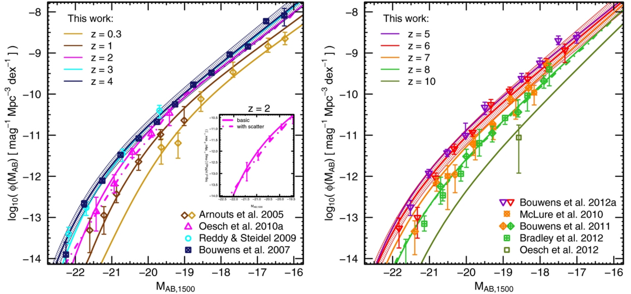
Figure 1. from A Physical Model for the 0 < z < 8 Redshift Evolution of the Galaxy Ultraviolet Luminosity and Stellar Mass Functions Tacchella, Trenti, & Carollo 2013 ApJL 768 L37 doi:10.1088/2041-8205/768/2/L37 https://dx.doi.org/10.1088/2041-8205/768/2/L37
