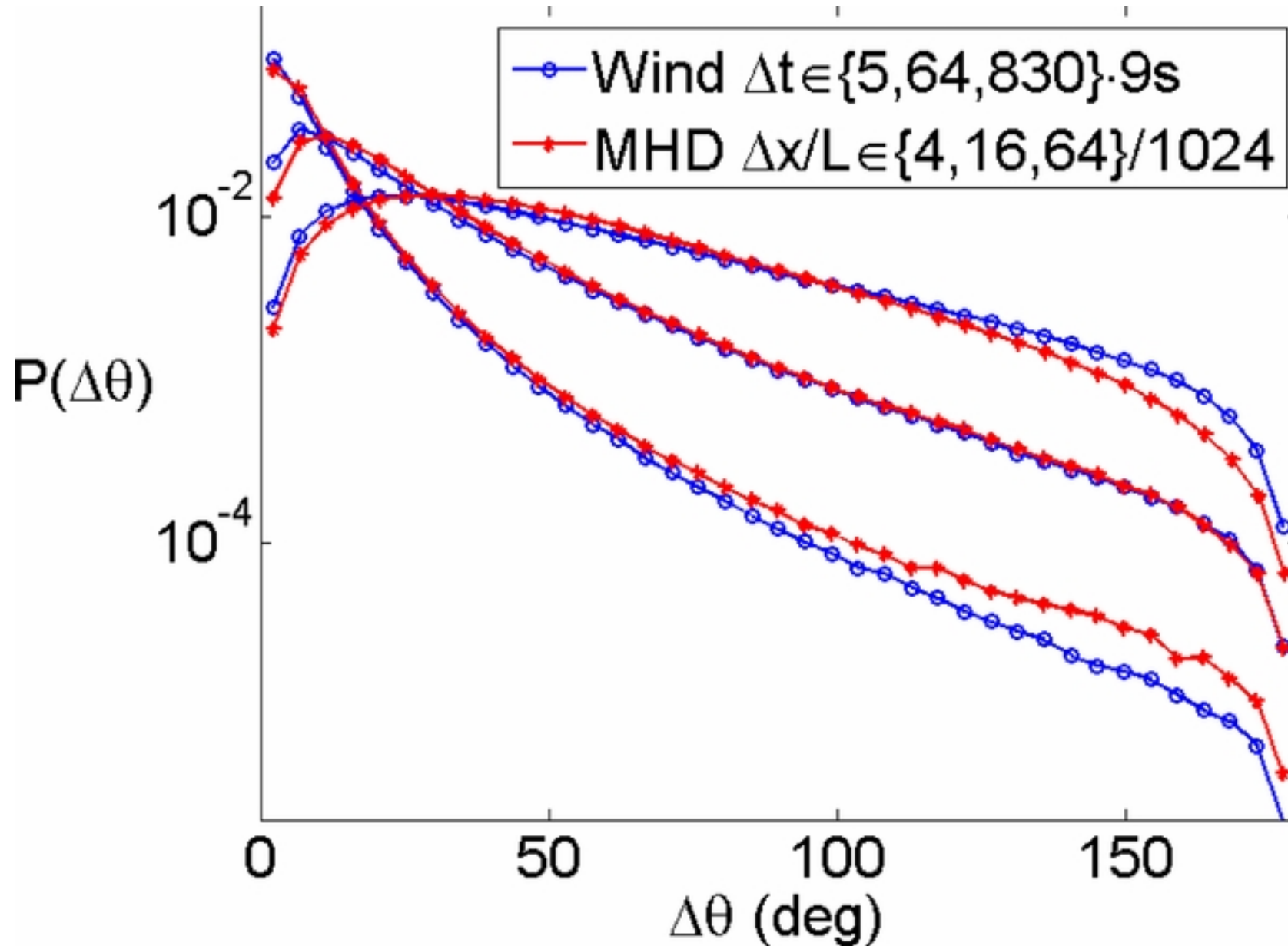
Figure 5. from Distribution of Magnetic Discontinuities in the Solar Wind and in Magnetohydrodynamic Turbulence Zhdankin, Boldyrev, & Mason 2012 ApJL 760 L22 doi:10.1088/2041-8205/760/2/L22 https://dx.doi.org/10.1088/2041-8205/760/2/L22 © 2012. The American Astronomical Society. All rights reserved.
