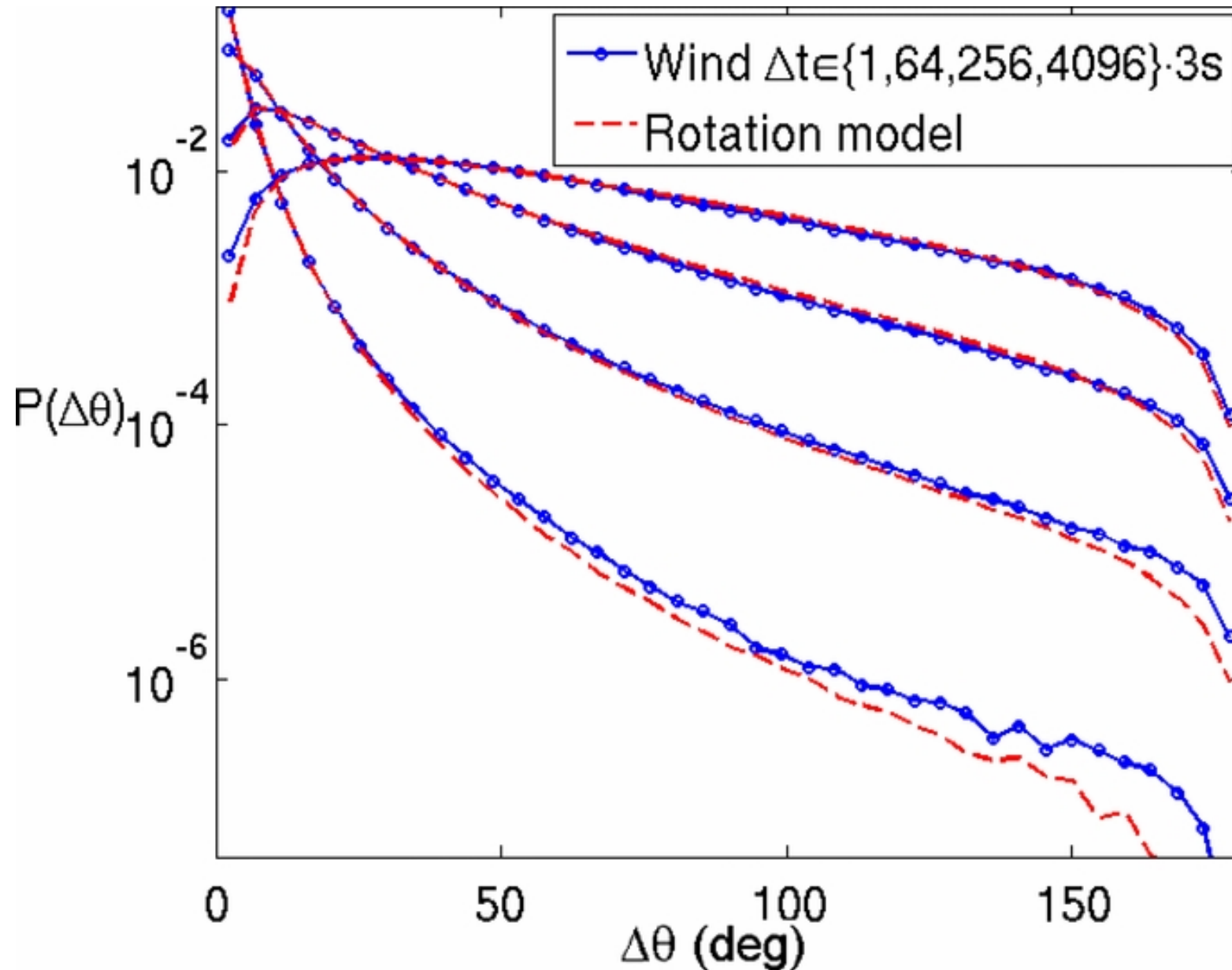
Figure 4. from Distribution of Magnetic Discontinuities in the Solar Wind and in Magnetohydrodynamic Turbulence Zhdankin, Boldyrev, & Mason 2012 ApJL 760 L22 doi:10.1088/2041-8205/760/2/L22 https://dx.doi.org/10.1088/2041-8205/760/2/L22 © 2012. The American Astronomical Society. All rights reserved.
