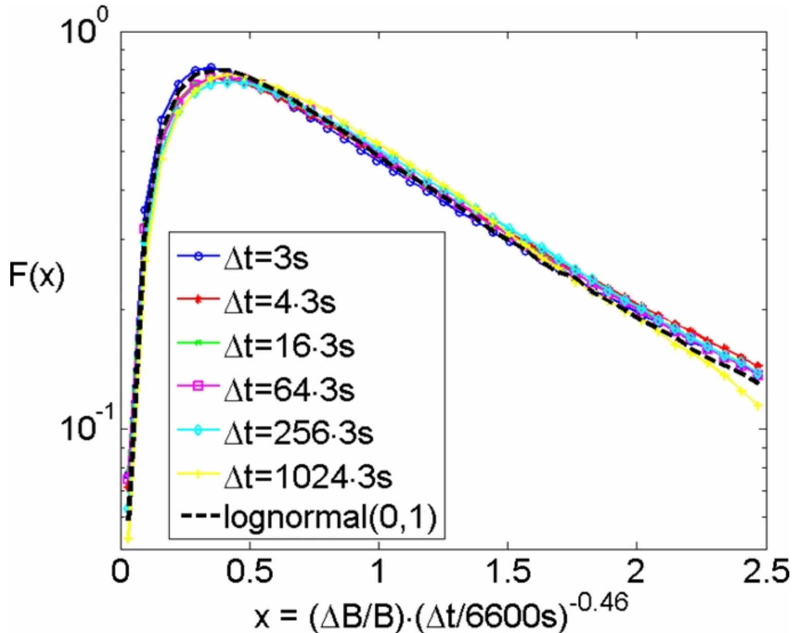
Figure 3. from Distribution of Magnetic Discontinuities in the Solar Wind and in Magnetohydrodynamic Turbulence Zhdankin, Boldyrev, & Mason 2012 ApJL 760 L22 doi:10.1088/2041-8205/760/2/L22 https://dx.doi.org/10.1088/2041-8205/760/2/L22 © 2012. The American Astronomical Society. All rights reserved.
