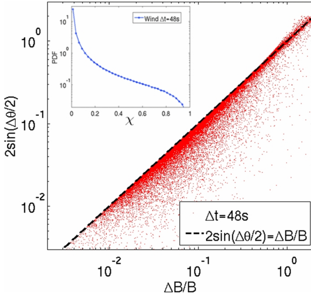
Figure 2. from Distribution of Magnetic Discontinuities in the Solar Wind and in Magnetohydrodynamic Turbulence Zhdankin, Boldyrev, & Mason 2012 ApJL 760 L22 doi:10.1088/2041-8205/760/2/L22 https://dx.doi.org/10.1088/2041-8205/760/2/L22 © 2012. The American Astronomical Society. All rights reserved.
