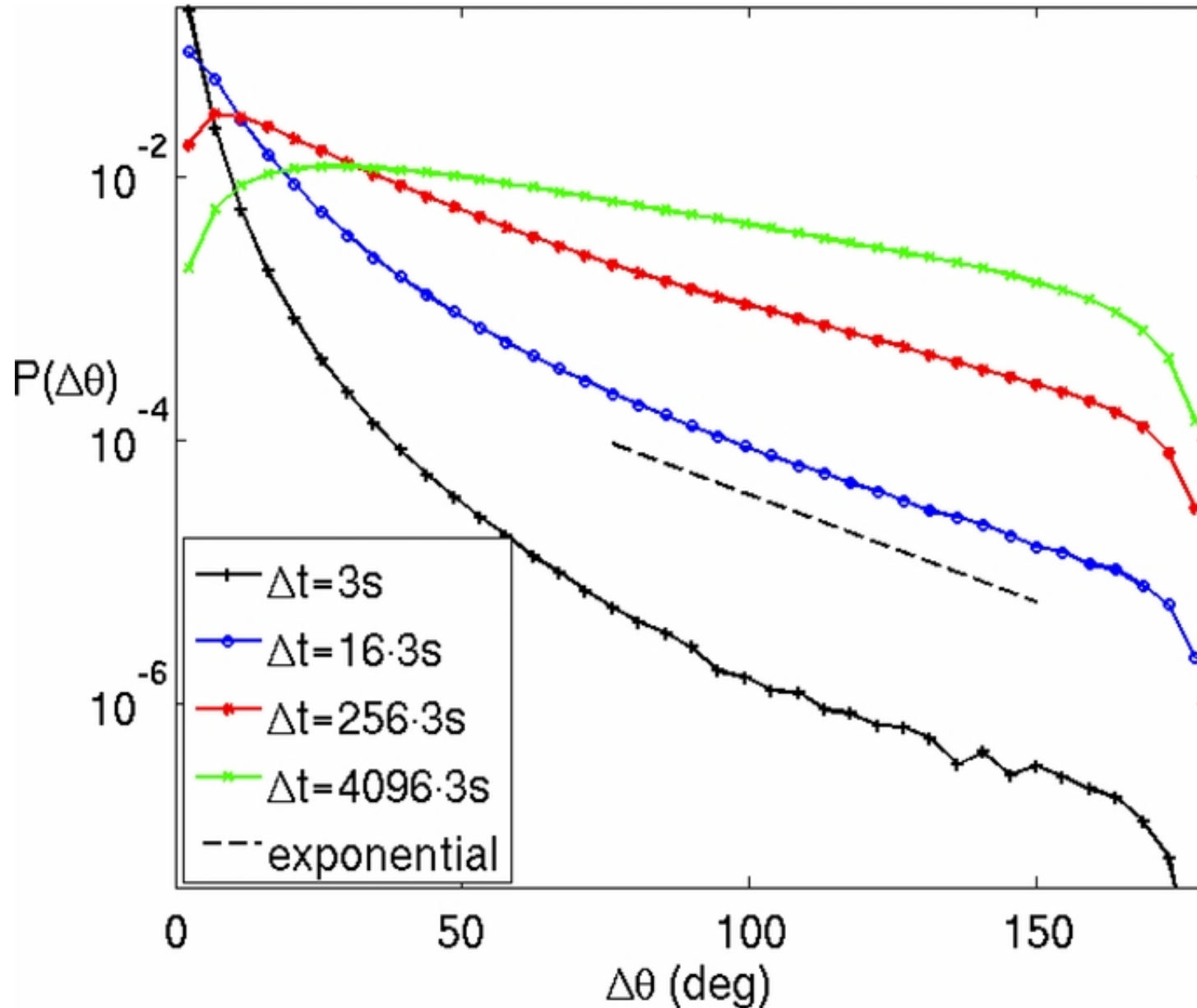
Figure 1. from Distribution of Magnetic Discontinuities in the Solar Wind and in Magnetohydrodynamic Turbulence Zhdankin, Boldyrev, & Mason 2012 ApJL 760 L22 doi:10.1088/2041-8205/760/2/L22 https://dx.doi.org/10.1088/2041-8205/760/2/L22 © 2012. The American Astronomical Society. All rights reserved.
