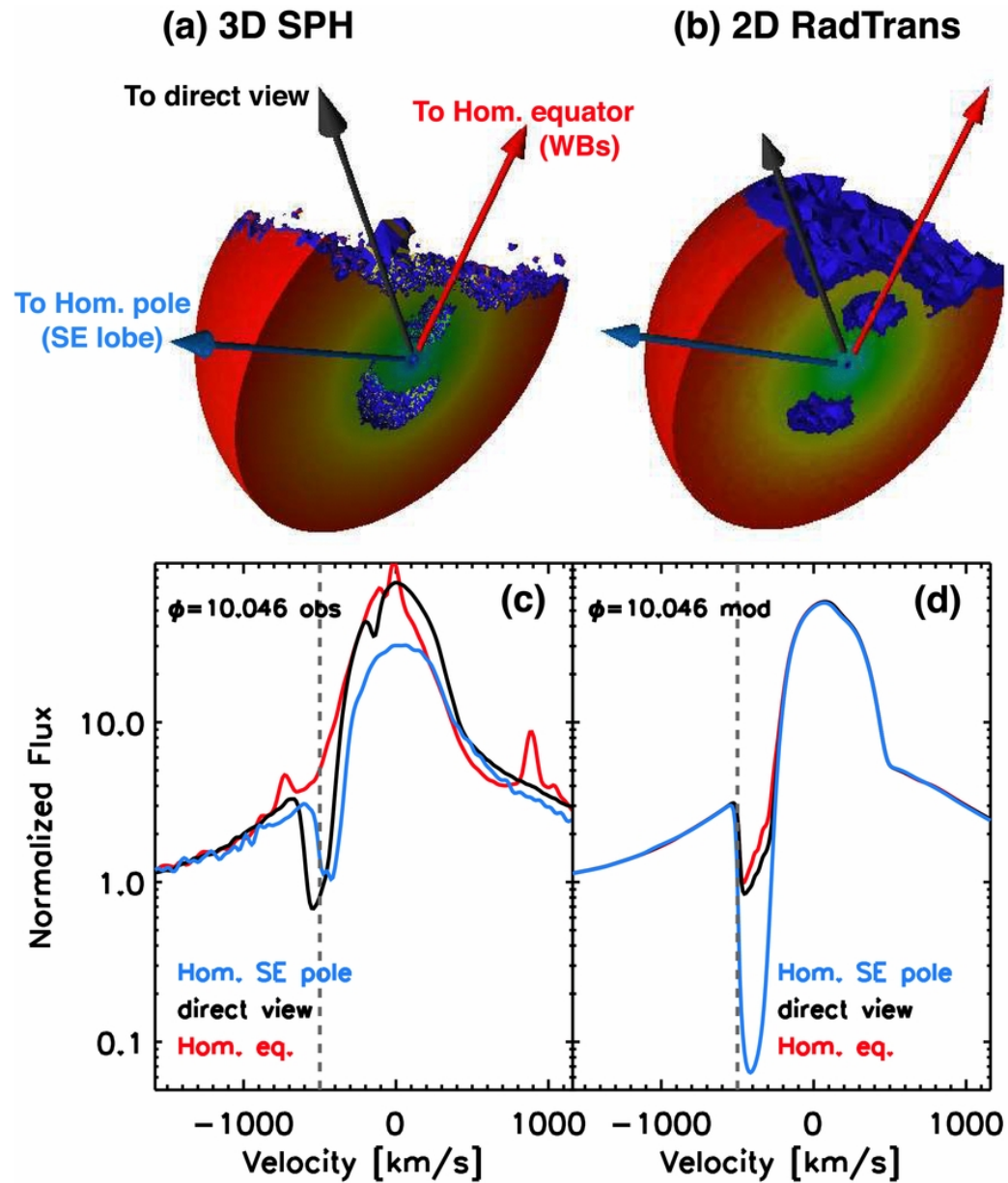
Figure 4. from A Companion as the Cause of Latitude-dependent Effects in the Wind of Eta Carinae Groh et al. 2012 ApJL 759 L2 doi:10.1088/2041-8205/759/1/L2 https://dx.doi.org/10.1088/2041-8205/759/1/L2 © 2012. The American Astronomical Society. All rights reserved.
