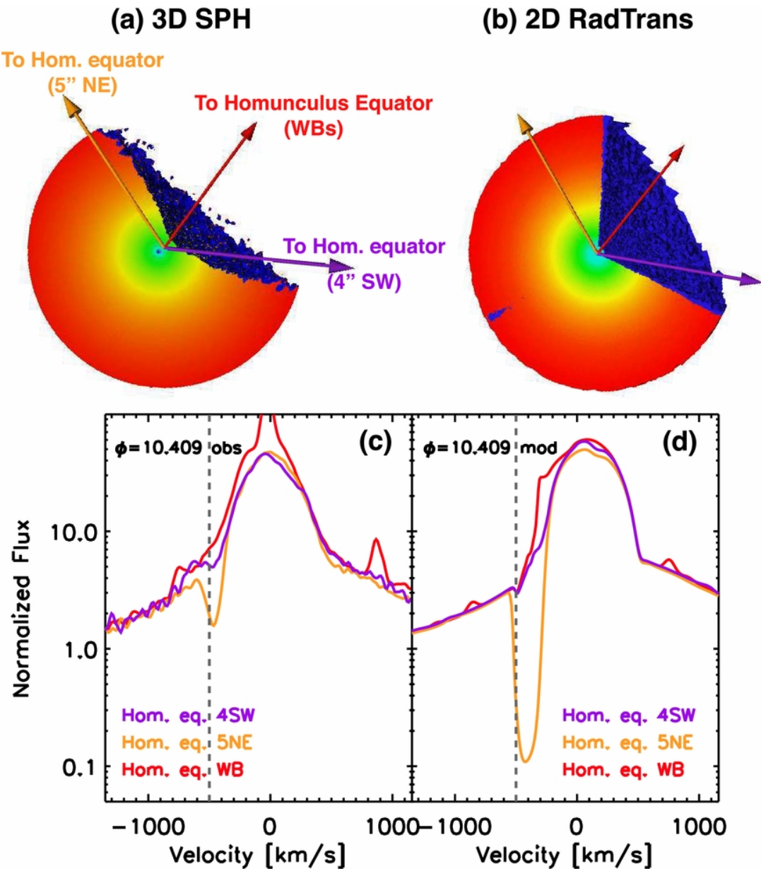
Figure 3. from A Companion as the Cause of Latitude-dependent Effects in the Wind of Eta Carinae Groh et al. 2012 ApJL 759 L2 doi:10.1088/2041-8205/759/1/L2 https://dx.doi.org/10.1088/2041-8205/759/1/L2 © 2012. The American Astronomical Society. All rights reserved.
