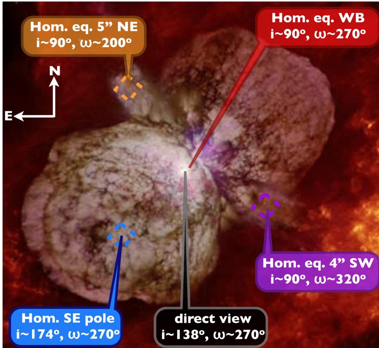
Figure 1. from A Companion as the Cause of Latitude-dependent Effects in the Wind of Eta Carinae Groh et al. 2012 ApJL 759 L2 doi:10.1088/2041-8205/759/1/L2 https://dx.doi.org/10.1088/2041-8205/759/1/L2 © 2012. The American Astronomical Society. All rights reserved.
