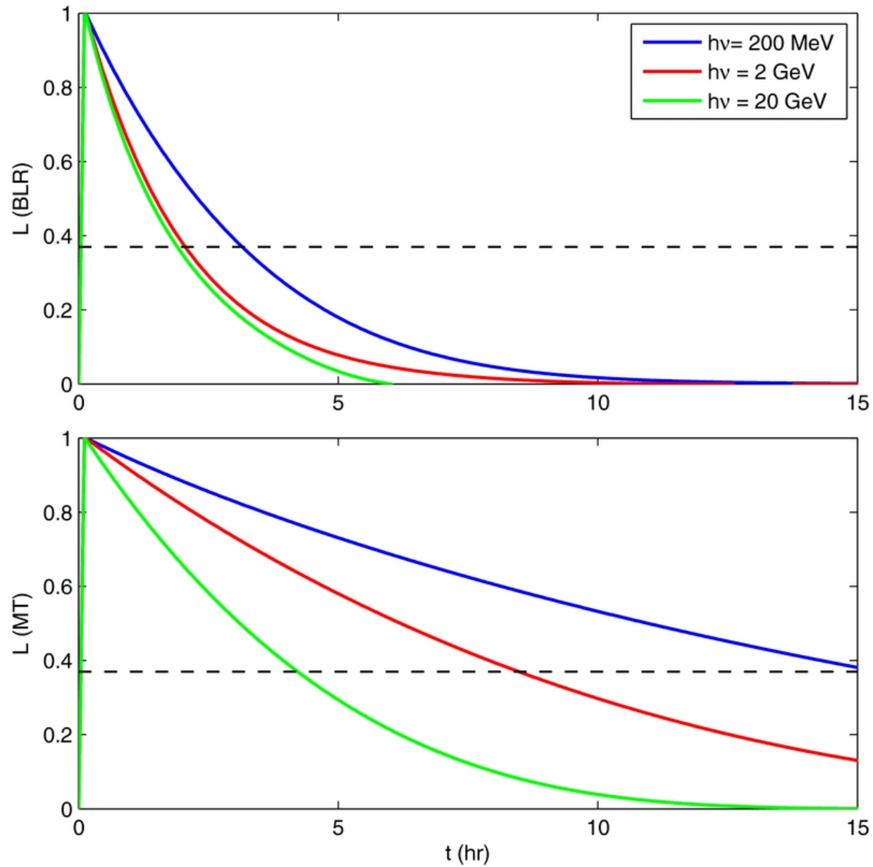
Figure 3. from A Method for Localizing Energy Dissipation in Blazars Using Fermi Variability Dotson et al. 2012 ApJL 758 L15 doi:10.1088/2041-8205/758/1/L15 https://dx.doi.org/10.1088/2041-8205/758/1/L15 © 2012. The American Astronomical Society. All rights reserved.
