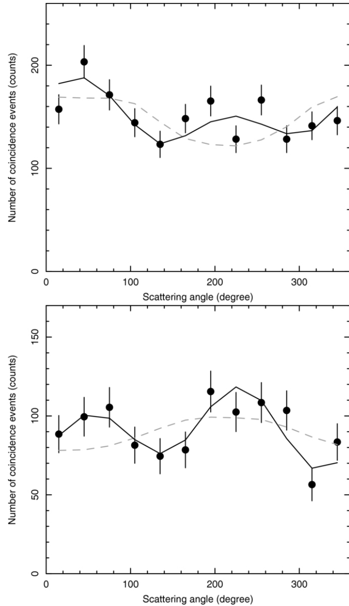
Figure 2. from Magnetic Structures in Gamma-Ray Burst Jets Probed by Gamma-Ray Polarization Yonetoku et al. 2012 ApJL 758 L1 doi:10.1088/2041-8205/758/1/L1 https://dx.doi.org/10.1088/2041-8205/758/1/L1 © 2012. The American Astronomical Society. All rights reserved.
