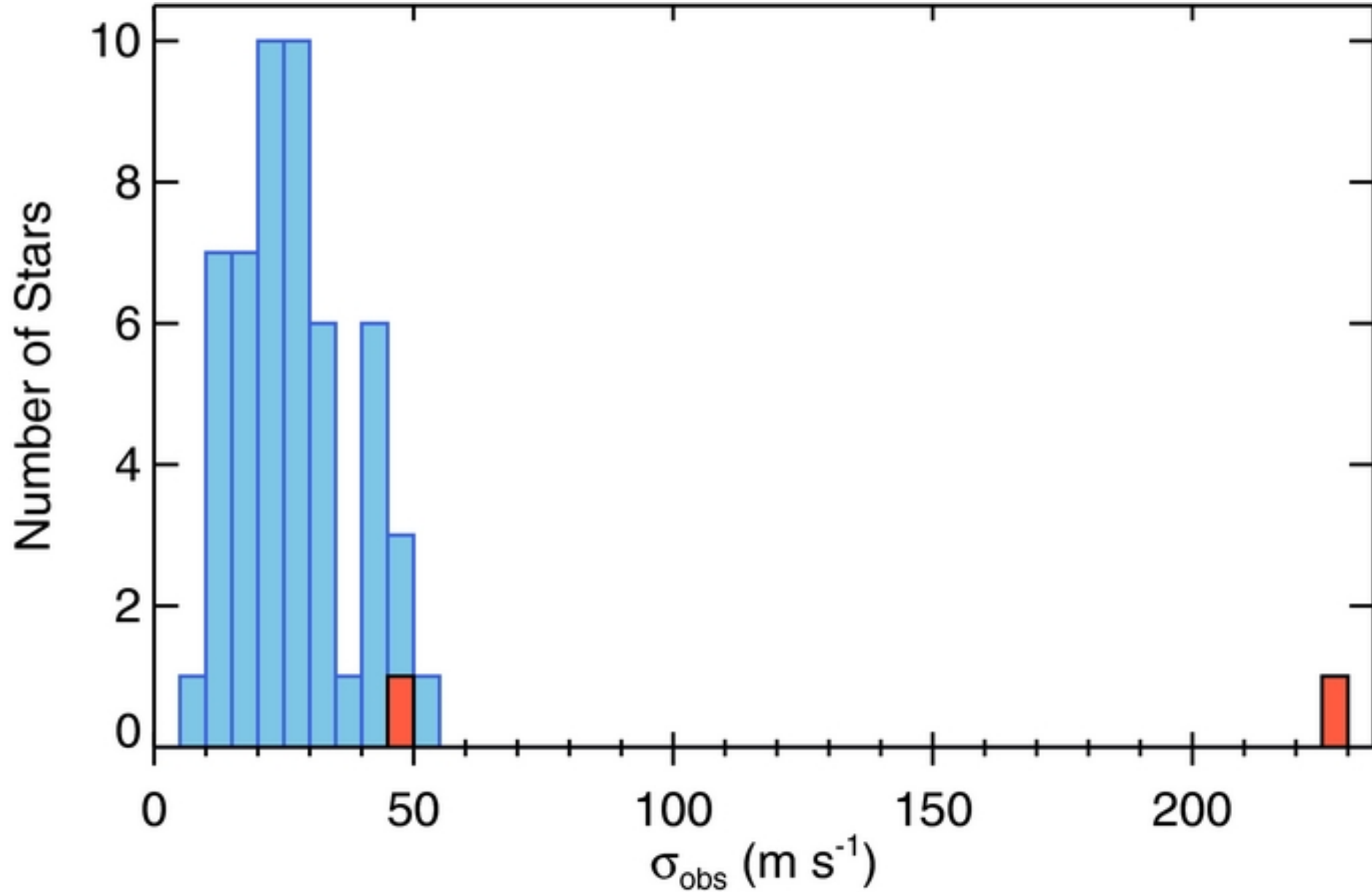
Figure 1. from Two “b”s in the Beehive: The Discovery of the First Hot Jupiters in an Open Cluster Quinn et al. 2012 ApJL 756 L33 doi:10.1088/2041-8205/756/2/L33 https://dx.doi.org/10.1088/2041-8205/756/2/L33 © 2012. The American Astronomical Society. All rights reserved.
