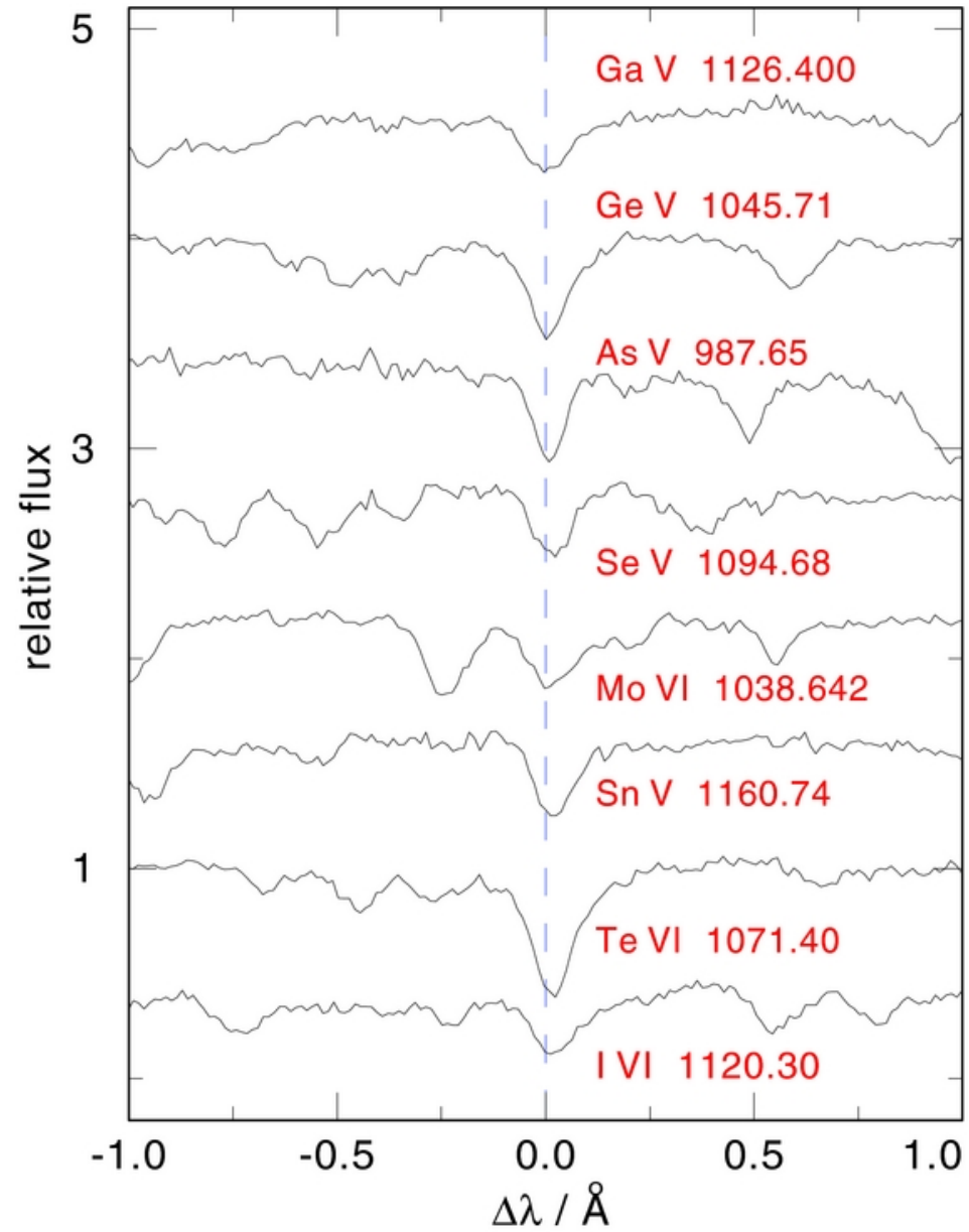
Figure 3. from First Detection of Krypton and Xenon in a White Dwarf Werner et al. 2012 ApJL 753 L7 doi:10.1088/2041-8205/753/1/L7 https://dx.doi.org/10.1088/2041-8205/753/1/L7 © 2012. The American Astronomical Society. All rights reserved.
