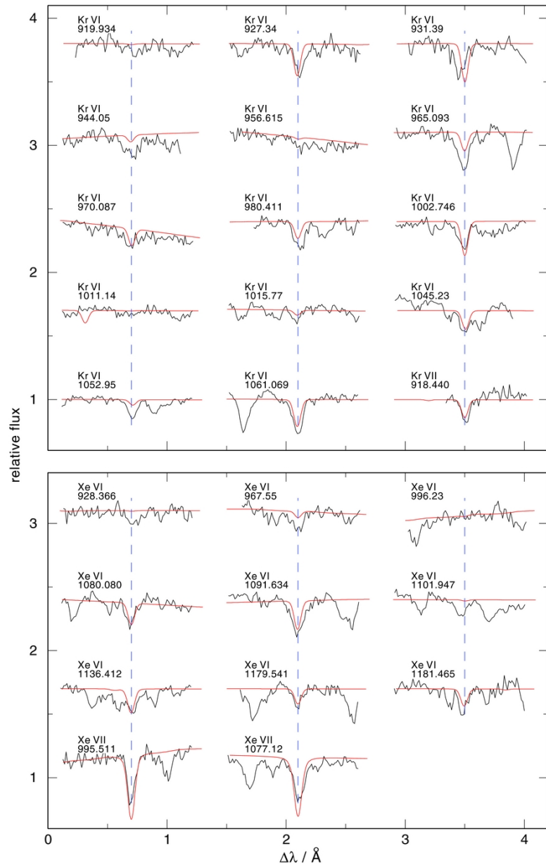
Figure 1. from First Detection of Krypton and Xenon in a White Dwarf Werner et al. 2012 ApJL 753 L7 doi:10.1088/2041-8205/753/1/L7 https://dx.doi.org/10.1088/2041-8205/753/1/L7 © 2012. The American Astronomical Society. All rights reserved.
