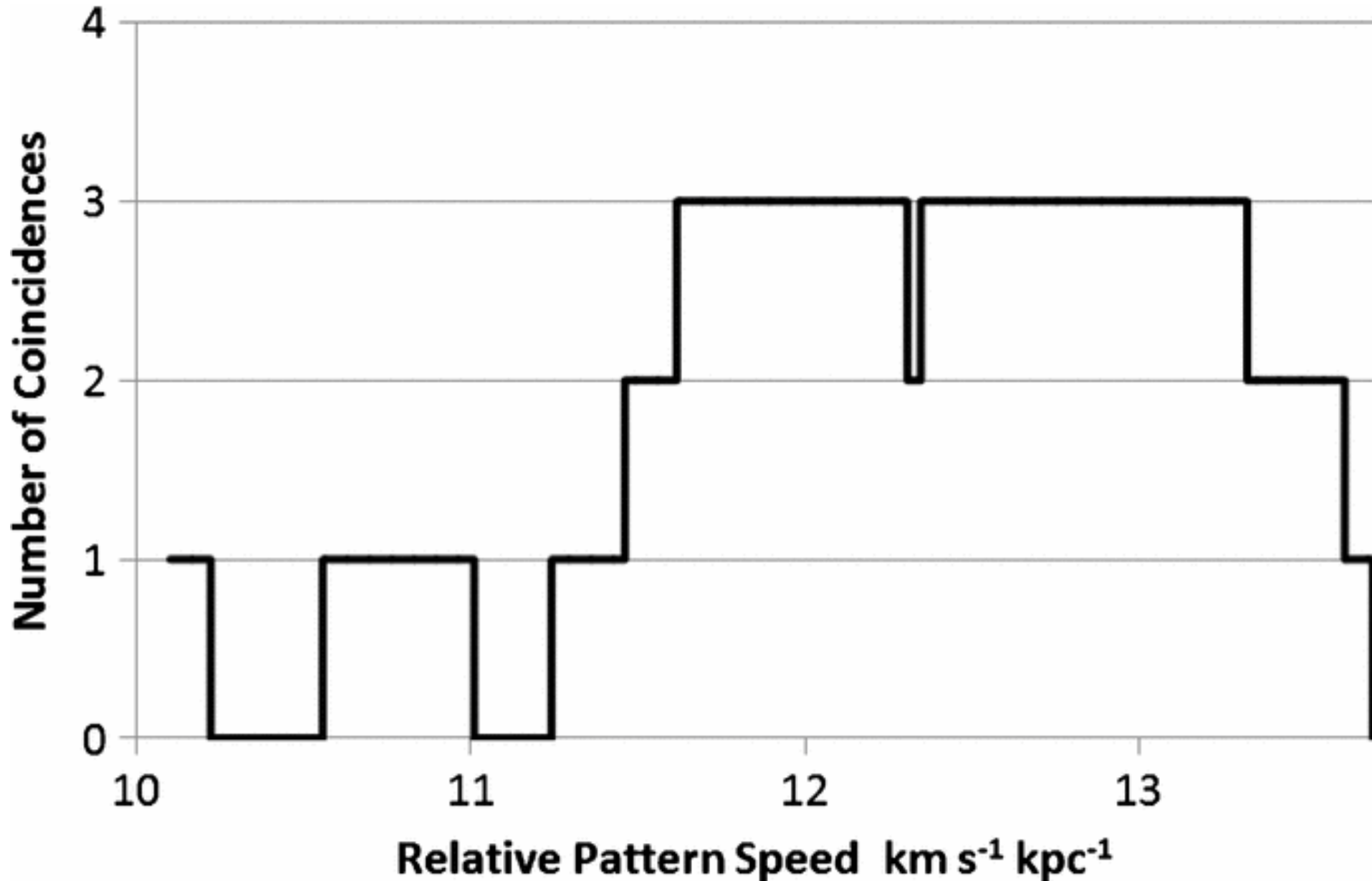
Figure 2. from Erratum: “Testing the Link between Terrestrial Climate Change and Galactic Spiral-arm Transit” (2009, ApJ, 705, l101) Erratum: 2009, ApJ, 705, L101 2012 ApJL 751 L45 doi:10.1088/2041-8205/751/2/L45 https://dx.doi.org/10.1088/2041-8205/751/2/L45 © 2012. The American Astronomical Society. All rights reserved.
