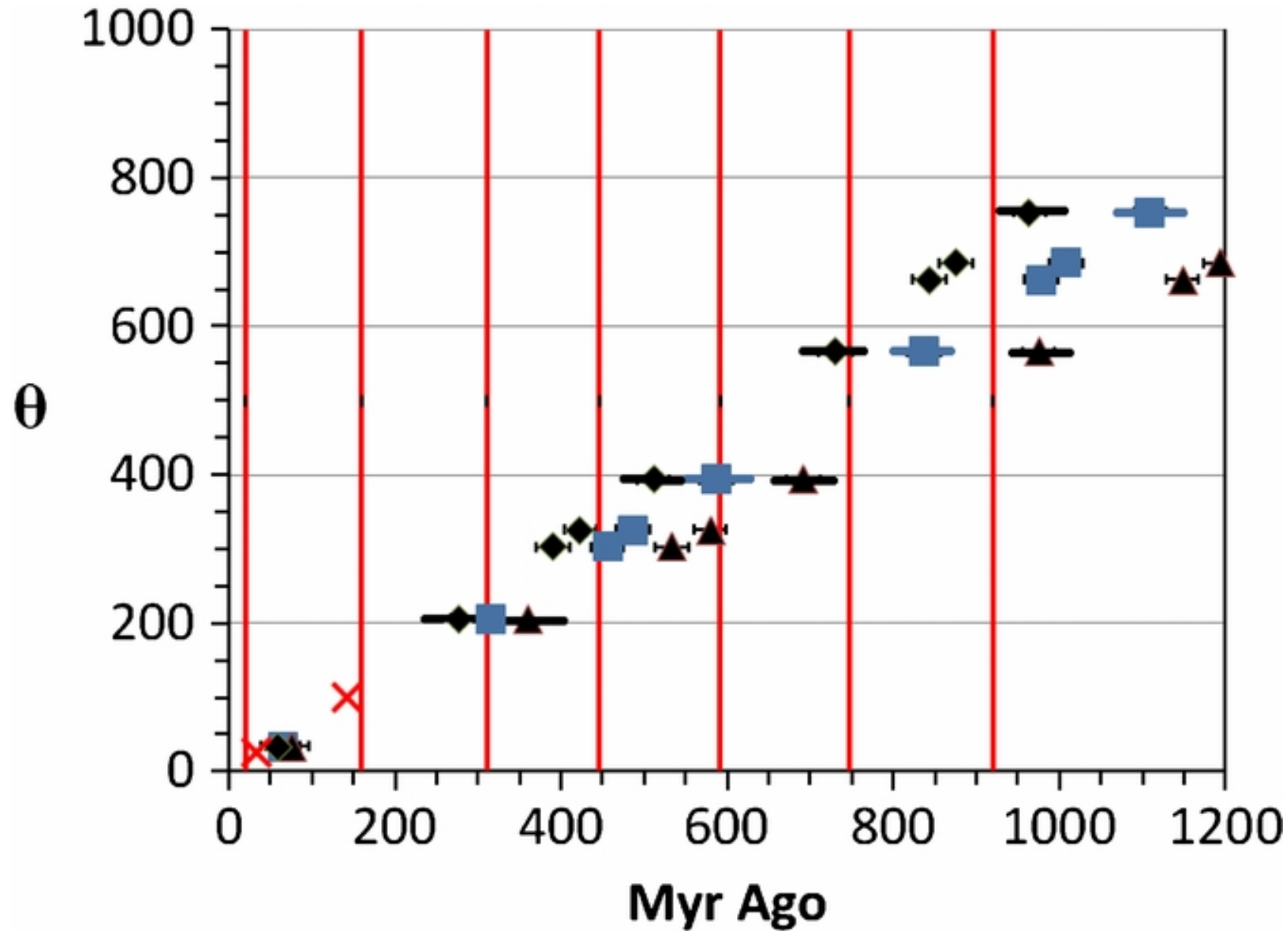
Figure 1. from Erratum: "Testing the Link between Terrestrial Climate Change and Galactic Spiral-arm Transit" (2009, ApJ, 705, l101) Erratum: 2009, ApJ, 705, L101 2012 ApJL 751 L45 doi:10.1088/2041-8205/751/2/L45 https://dx.doi.org/10.1088/2041-8205/751/2/L45 © 2012. The American Astronomical Society. All rights reserved.
