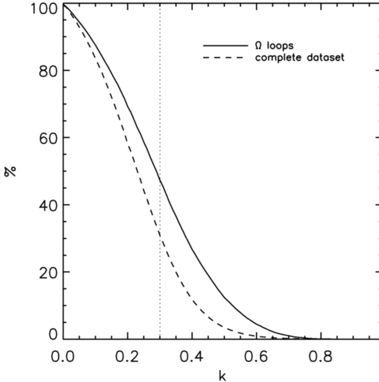
Figure 3. from On the Polarimetric Signature of Emerging Magnetic Loops in the Quiet Sun Vitichí 2012 ApJL 747 L36 doi:10.1088/2041-8205/747/2/L36 https://dx.doi.org/10.1088/2041-8205/747/2/L36 © 2012. The American Astronomical Society. All rights reserved.
