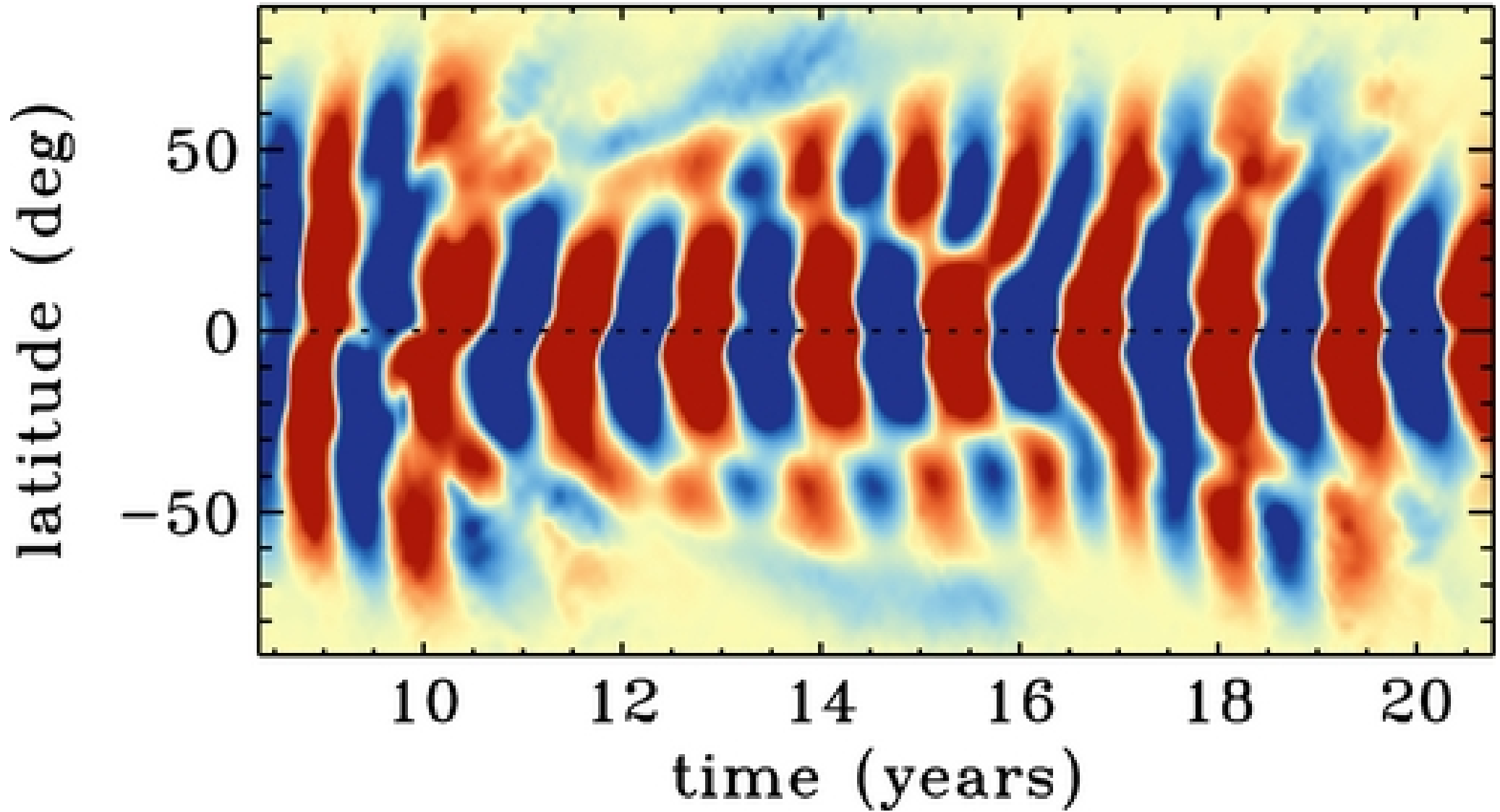
Figure 4. from Convective Babcock-Leighton Dynamo Models Miesch & Brown 2012 ApJL 746 L26 doi:10.1088/2041-8205/746/2/L26 https://dx.doi.org/10.1088/2041-8205/746/2/L26 © 2012. The American Astronomical Society. All rights reserved.
