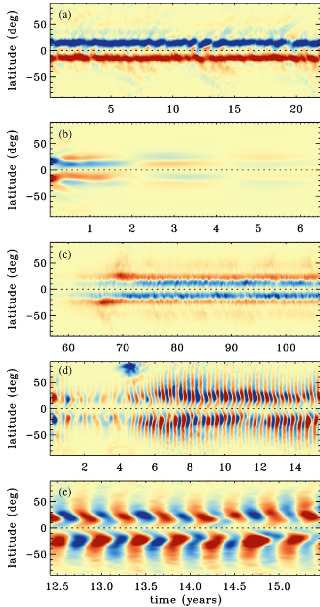
Figure 2. from Convective Babcock-Leighton Dynamo Models Miesch & Brown 2012 ApJL 746 L26 doi:10.1088/2041-8205/746/2/L26 https://dx.doi.org/10.1088/2041-8205/746/2/L26 © 2012. The American Astronomical Society. All rights reserved.
