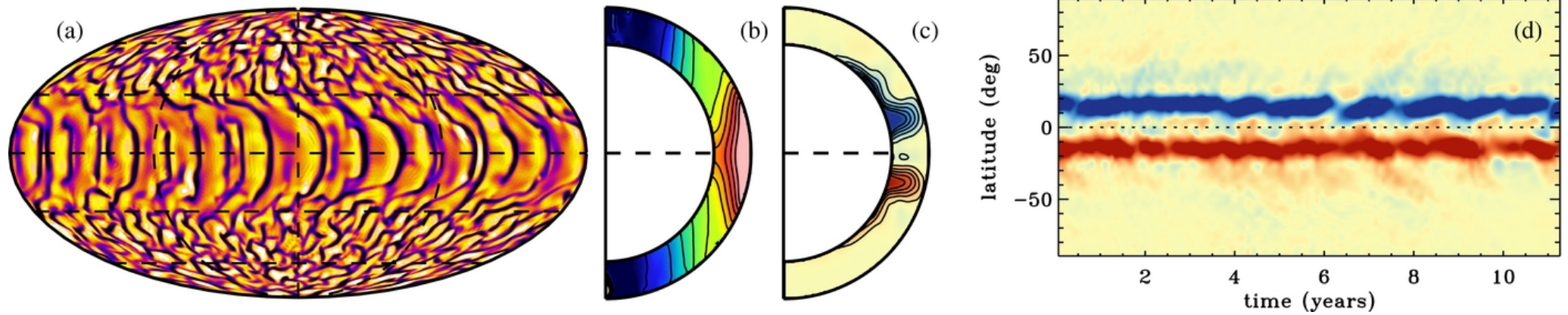
Figure 1. from Convective Babcock-Leighton Dynamo Models Miesch & Brown 2012 ApJL 746 L26 doi:10.1088/2041-8205/746/2/L26 https://dx.doi.org/10.1088/2041-8205/746/2/L26 © 2012. The American Astronomical Society. All rights reserved.
