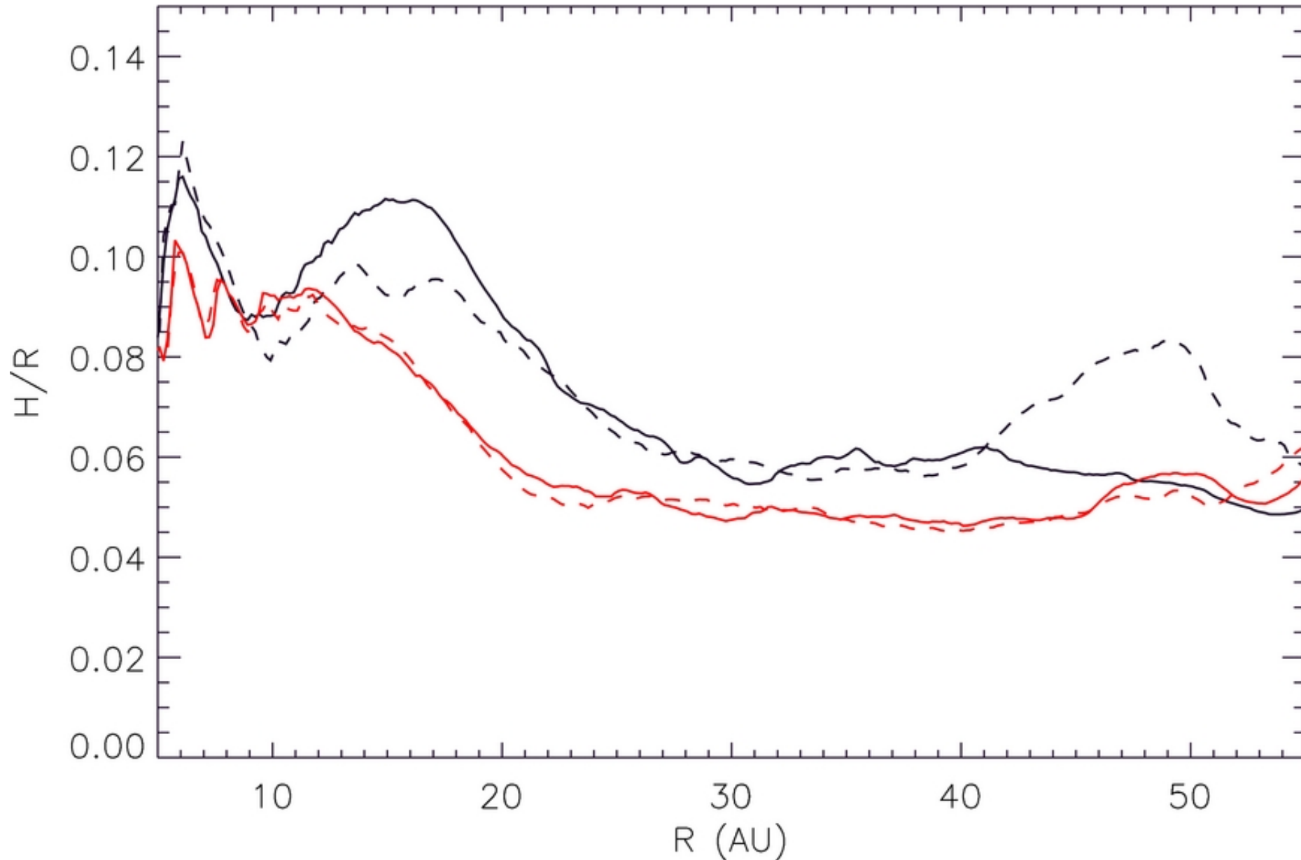
Figure 4. from Migration of Gas Giant Planets in Gravitationally Unstable Disks Michael, Durisen, & Boley 2011 ApJL 737 L42 doi:10.1088/2041-8205/737/2/L42 https://dx.doi.org/10.1088/2041-8205/737/2/L42 © 2011. The American Astronomical Society. All rights reserved.
