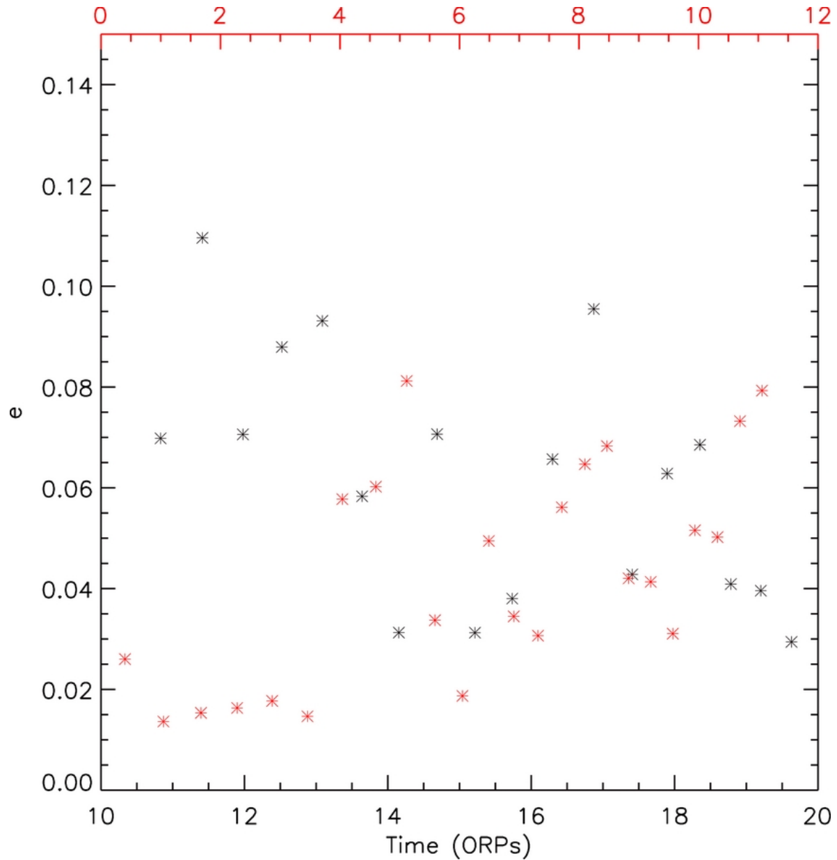
Figure 3. from Migration of Gas Giant Planets in Gravitationally Unstable Disks Michael, Durisen, & Boley 2011 ApJL 737 L42 doi:10.1088/2041-8205/737/2/L42 https://dx.doi.org/10.1088/2041-8205/737/2/L42
