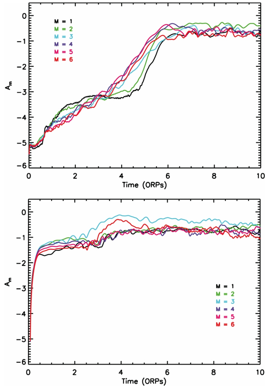
Figure 1. from Migration of Gas Giant Planets in Gravitationally Unstable Disks Michael, Durisen, & Boley 2011 ApJL 737 L42 doi:10.1088/2041-8205/737/2/L42 https://dx.doi.org/10.1088/2041-8205/737/2/L42 © 2011. The American Astronomical Society. All rights reserved.
