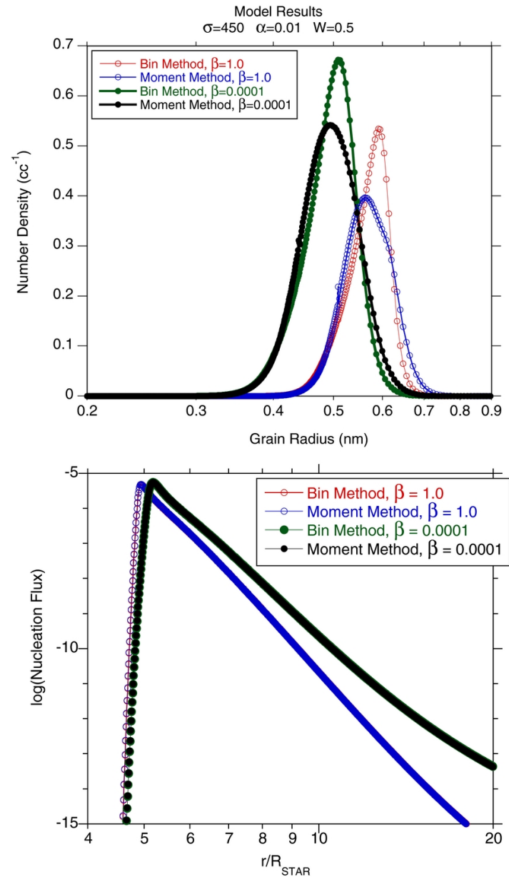
Figure 1. from The Lack of Chemical Equilibrium does not Preclude the use of Classical Nucleation Theory in Circumstellar Outflows Paquette & Nuth iii 2011 ApJL 737 L6 doi:10.1088/2041-8205/737/1/L6 https://dx.doi.org/10.1088/2041-8205/737/1/L6 © 2011. The American Astronomical Society. All rights reserved.
