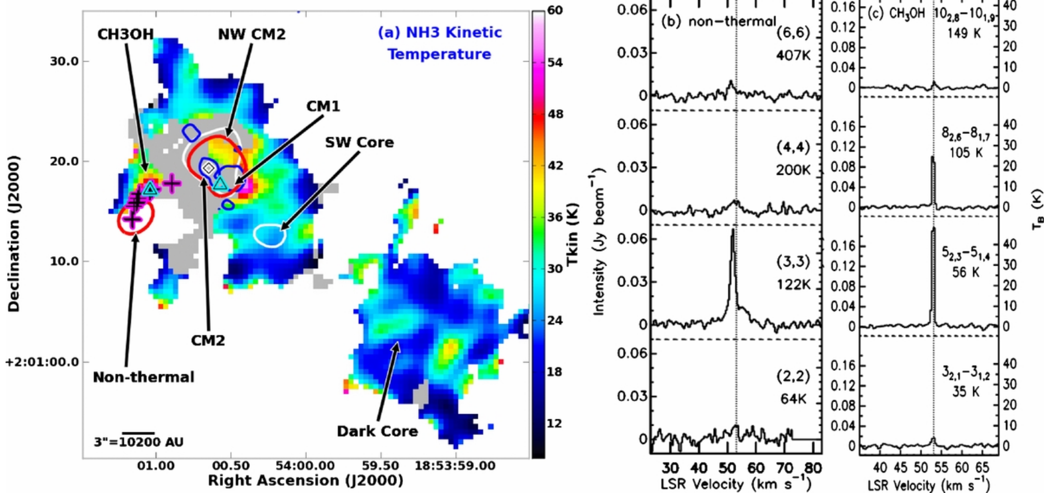
Figure 3. from First Results from a 1.3 cm Expanded Very Large Array Survey of Massive Protostellar Objects: G35.03+0.35 Brogan et al. 2011 ApJL 739 L16 doi:10.1088/2041-8205/739/1/L16 https://dx.doi.org/10.1088/2041-8205/739/1/L16 © 2011. The American Astronomical Society. All rights reserved.
