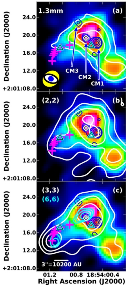
Figure 2. from First Results from a 1.3 cm Expanded Very Large Array Survey of Massive Protostellar Objects: G35.03+0.35 Brogan et al. 2011 ApJL 739 L16 doi:10.1088/2041-8205/739/1/L16 https://dx.doi.org/10.1088/2041-8205/739/1/L16 © 2011. The American Astronomical Society. All rights reserved.
