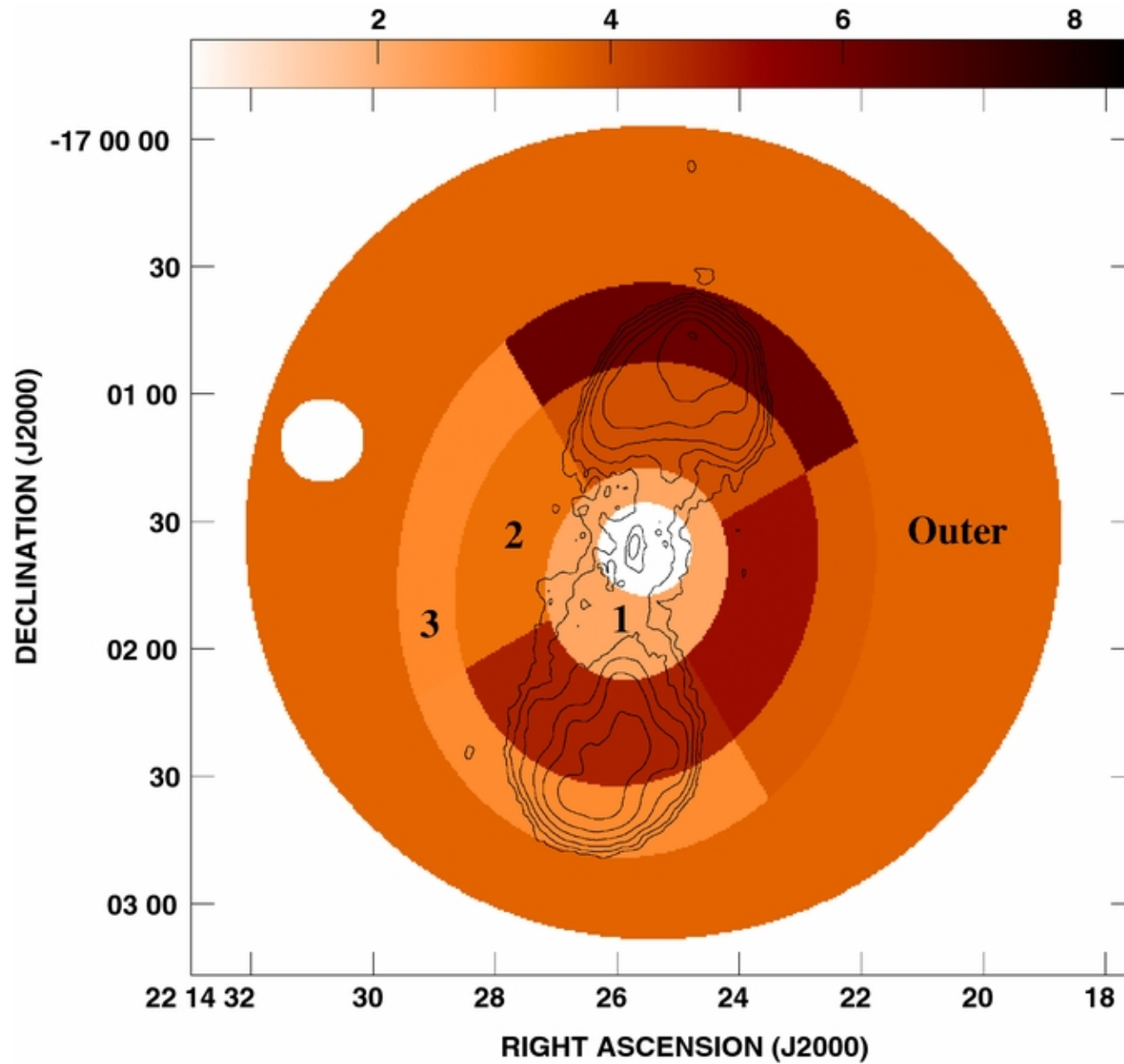
Figure 3. from A Large-scale Shock Surrounding a Powerful Radio Galaxy? Croston et al. 2011 ApJL 734 L28 doi:10.1088/2041-8205/734/2/L28 https://dx.doi.org/10.1088/2041-8205/734/2/L28 © 2011. The American Astronomical Society. All rights reserved.
