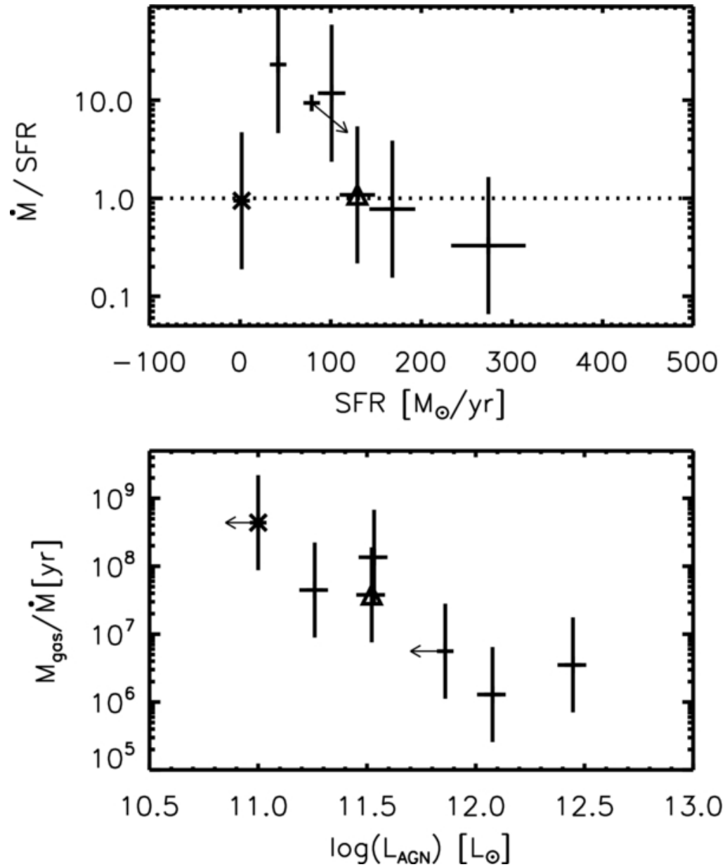
Figure 3. from Massive Molecular Outflows and Negative Feedback in ULIRGs Observed by Herschel-PACS Sturm et al. 2011 ApJL 733 L16 doi:10.1088/2041-8205/733/1/L16 https://dx.doi.org/10.1088/2041-8205/733/1/L16 © 2011. The American Astronomical Society. All rights reserved.
