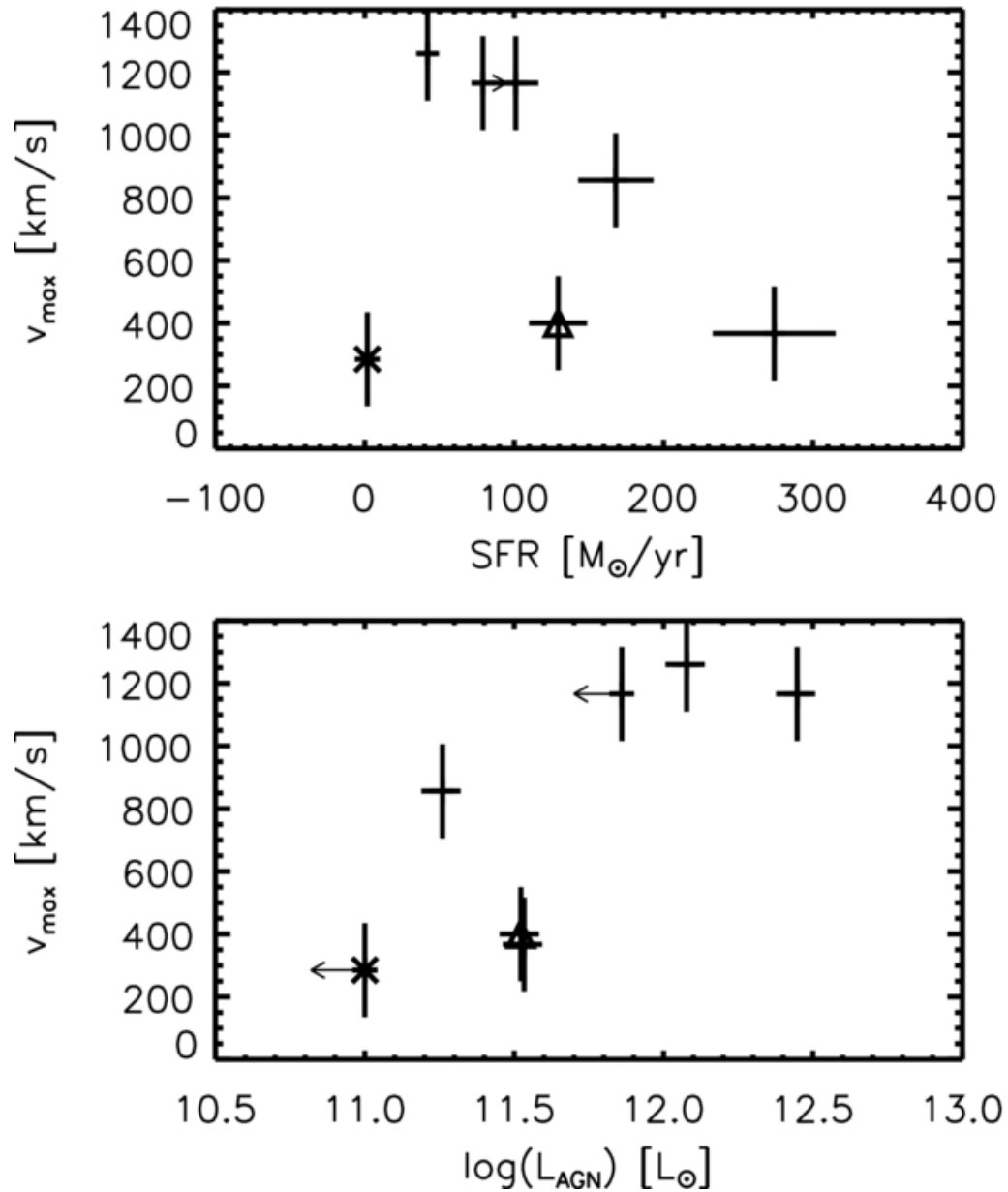
Figure 2. from Massive Molecular Outflows and Negative Feedback in ULIRGs Observed by Herschel-PACS Sturm et al. 2011 ApJL 733 L16 doi:10.1088/2041-8205/733/1/L16 https://dx.doi.org/10.1088/2041-8205/733/1/L16 © 2011. The American Astronomical Society. All rights reserved.
