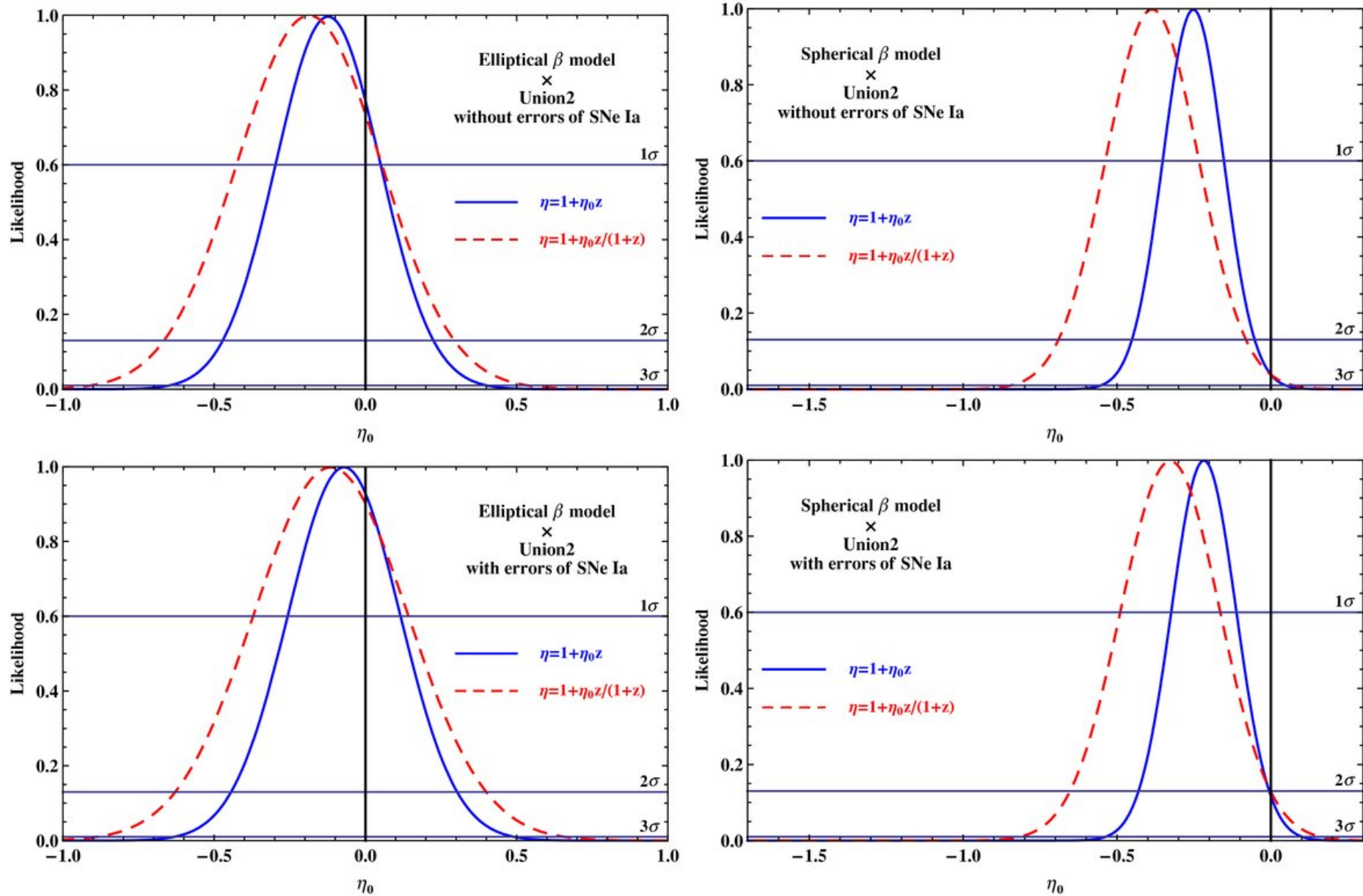
Figure 3. from Cosmological-model-independent Tests for the Distance–Duality Relation from Galaxy Clusters and Type Ia Supernova Li, Wu, & Yu 2011 ApJL 729 L14 doi:10.1088/2041-8205/729/1/L14 https://dx.doi.org/10.1088/2041-8205/729/1/L14 © 2011. The American Astronomical Society. All rights reserved.
