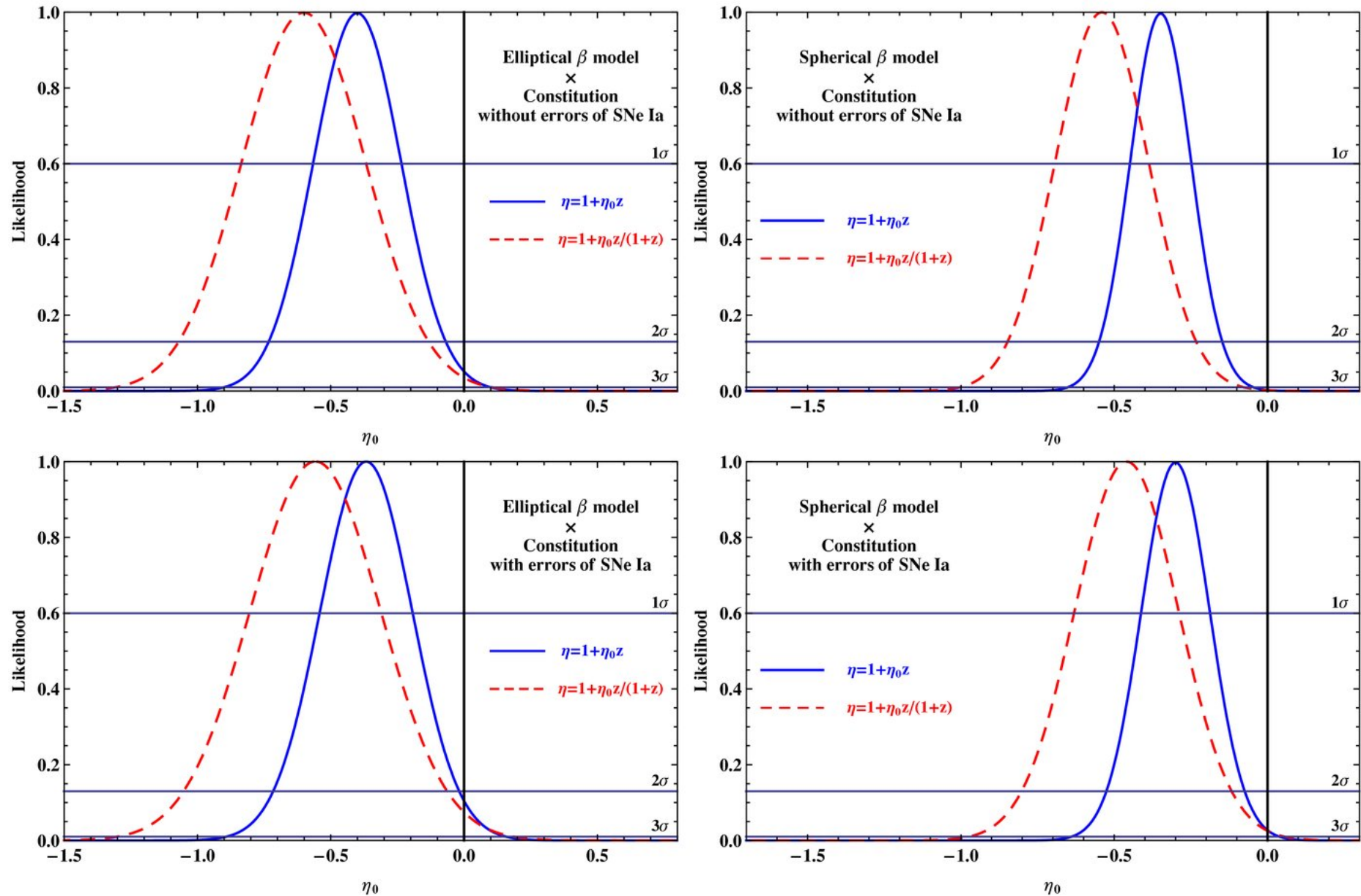
Figure 2. from Cosmological-model-independent Tests for the Distance–Duality Relation from Galaxy Clusters and Type Ia Supernova Li, Wu, & Yu 2011 ApJL 729 L14 doi:10.1088/2041-8205/729/1/L14 https://dx.doi.org/10.1088/2041-8205/729/1/L14 © 2011. The American Astronomical Society. All rights reserved.
