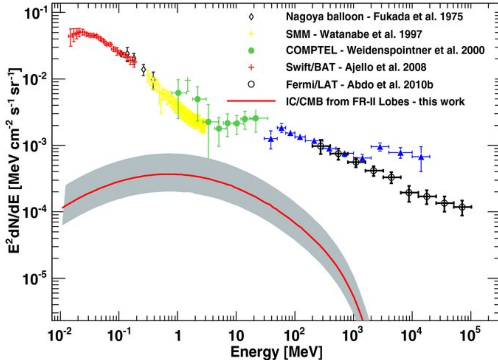
Figure 3. from Fueling Lobes of Radio Galaxies: Statistical Particle Acceleration and the Extragalactic -ray Background Massaro & Ajello 2011 ApJL 729 L12 doi:10.1088/2041-8205/729/1/L12 https://dx.doi.org/10.1088/2041-8205/729/1/L12 © 2011. The American Astronomical Society. All rights reserved.
