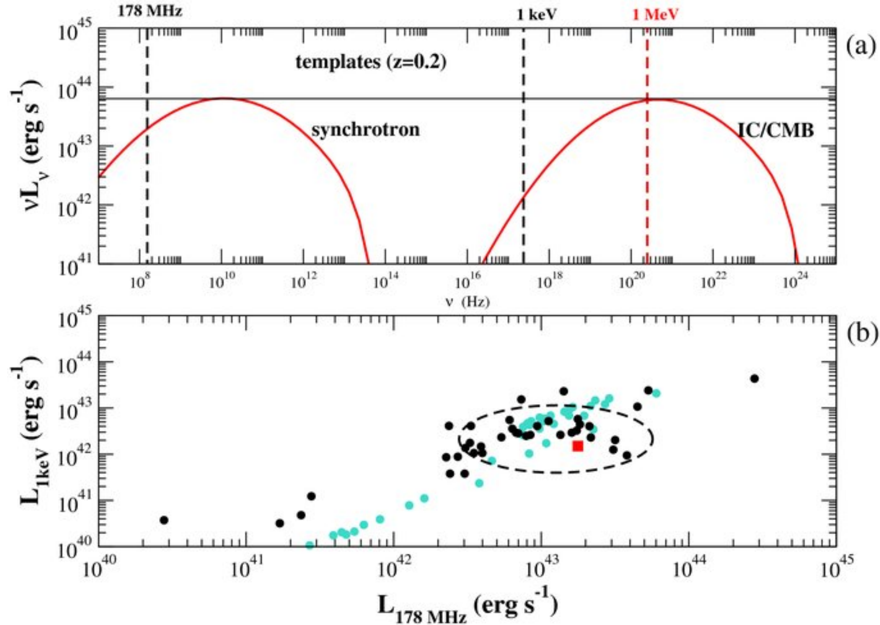
Figure 2. from Fueling Lobes of Radio Galaxies: Statistical Particle Acceleration and the Extragalactic -ray Background Massaro & Ajello 2011 ApJL 729 L12 doi:10.1088/2041-8205/729/1/L12 https://dx.doi.org/10.1088/2041-8205/729/1/L12 © 2011. The American Astronomical Society. All rights reserved.
