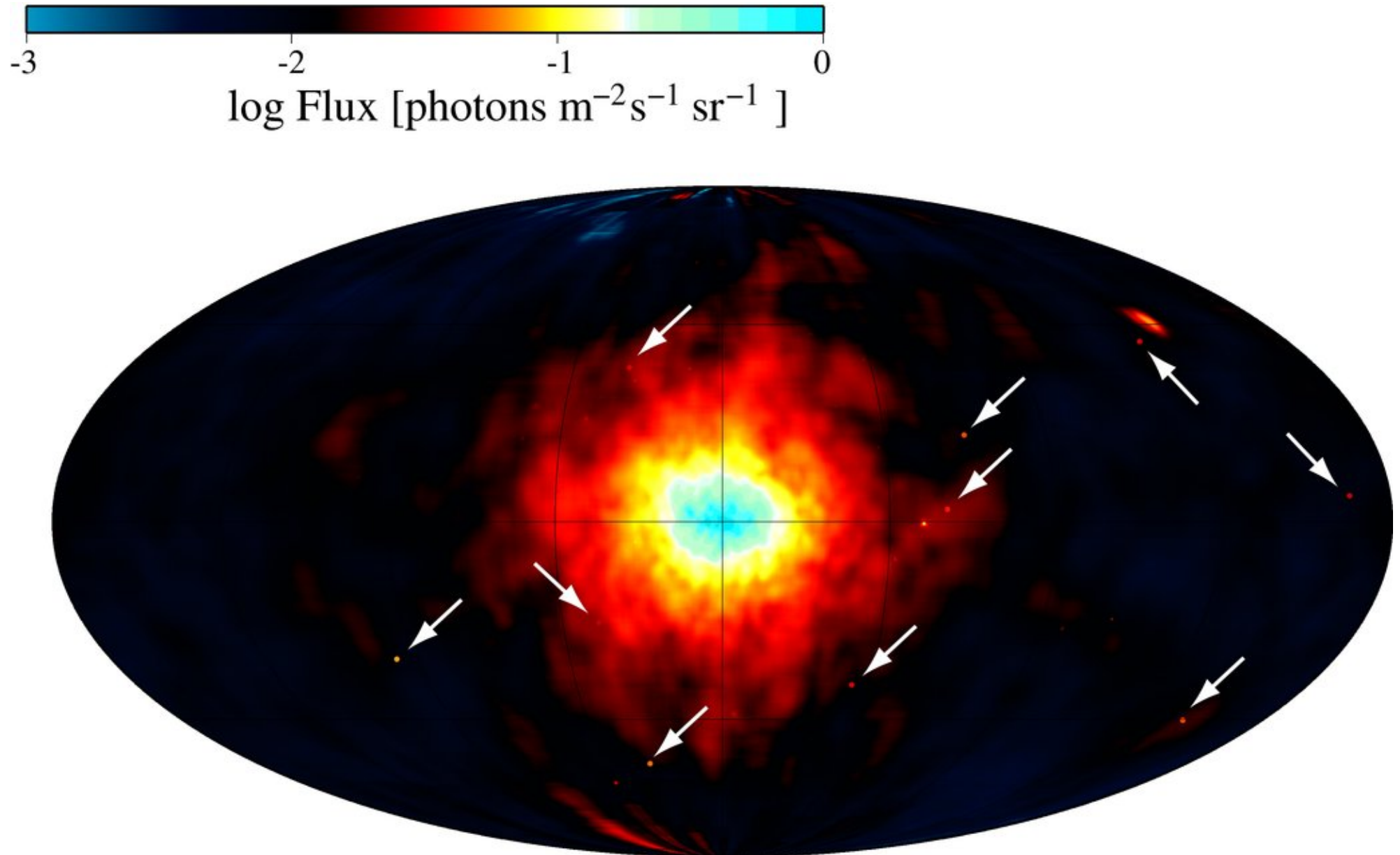
Figure 5. from Gamma-ray Signal from Earth-mass Dark Matter Microhalos ISHIYAMA, MAKINO, & EBISUZAKI 2010 ApJL 723 L195 doi:10.1088/2041-8205/723/2/L195 https://dx.doi.org/10.1088/2041-8205/723/2/L195 © 2010. The American Astronomical Society. All rights reserved.
