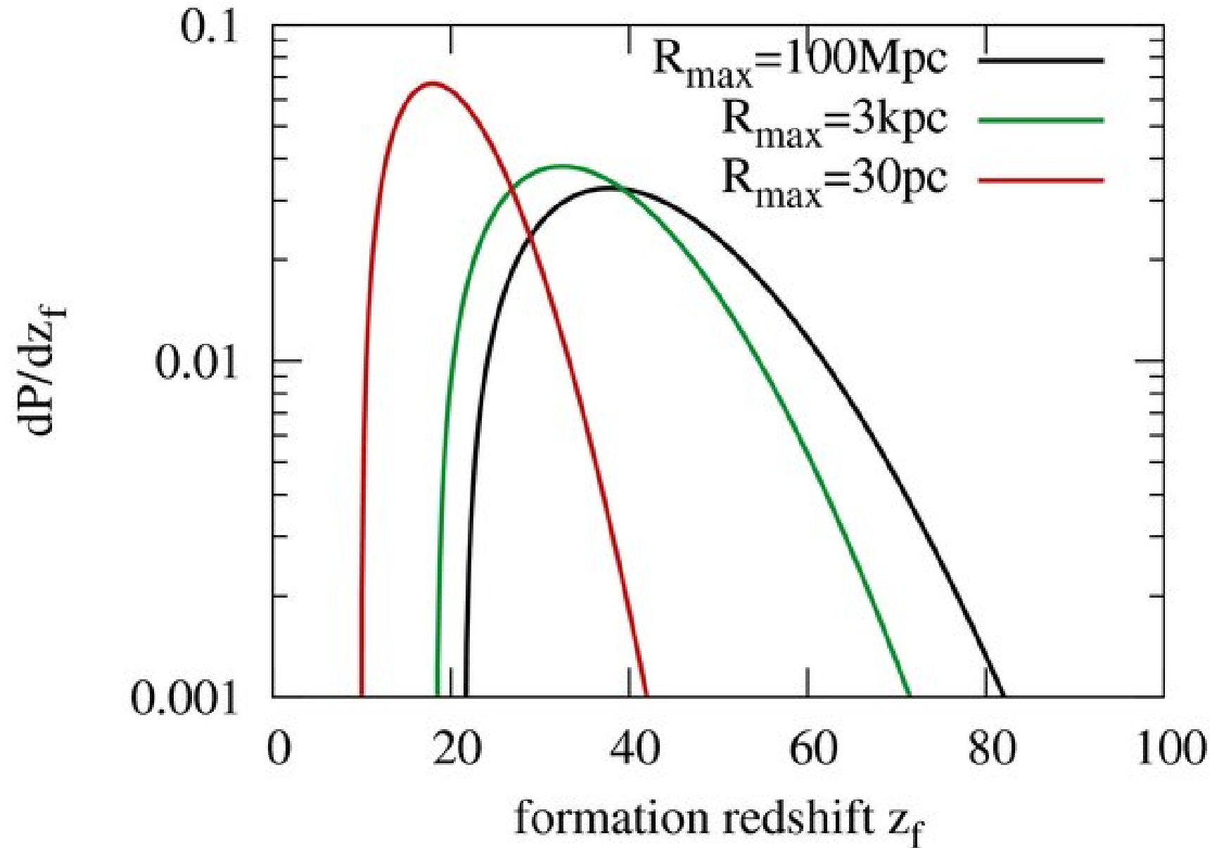
Figure 3. from Gamma-ray Signal from Earth-mass Dark Matter Microhalos ISHIYAMA, MAKINO, & EBISUZAKI 2010 ApJL 723 L195 doi:10.1088/2041-8205/723/2/L195 https://dx.doi.org/10.1088/2041-8205/723/2/L195 © 2010. The American Astronomical Society. All rights reserved.
