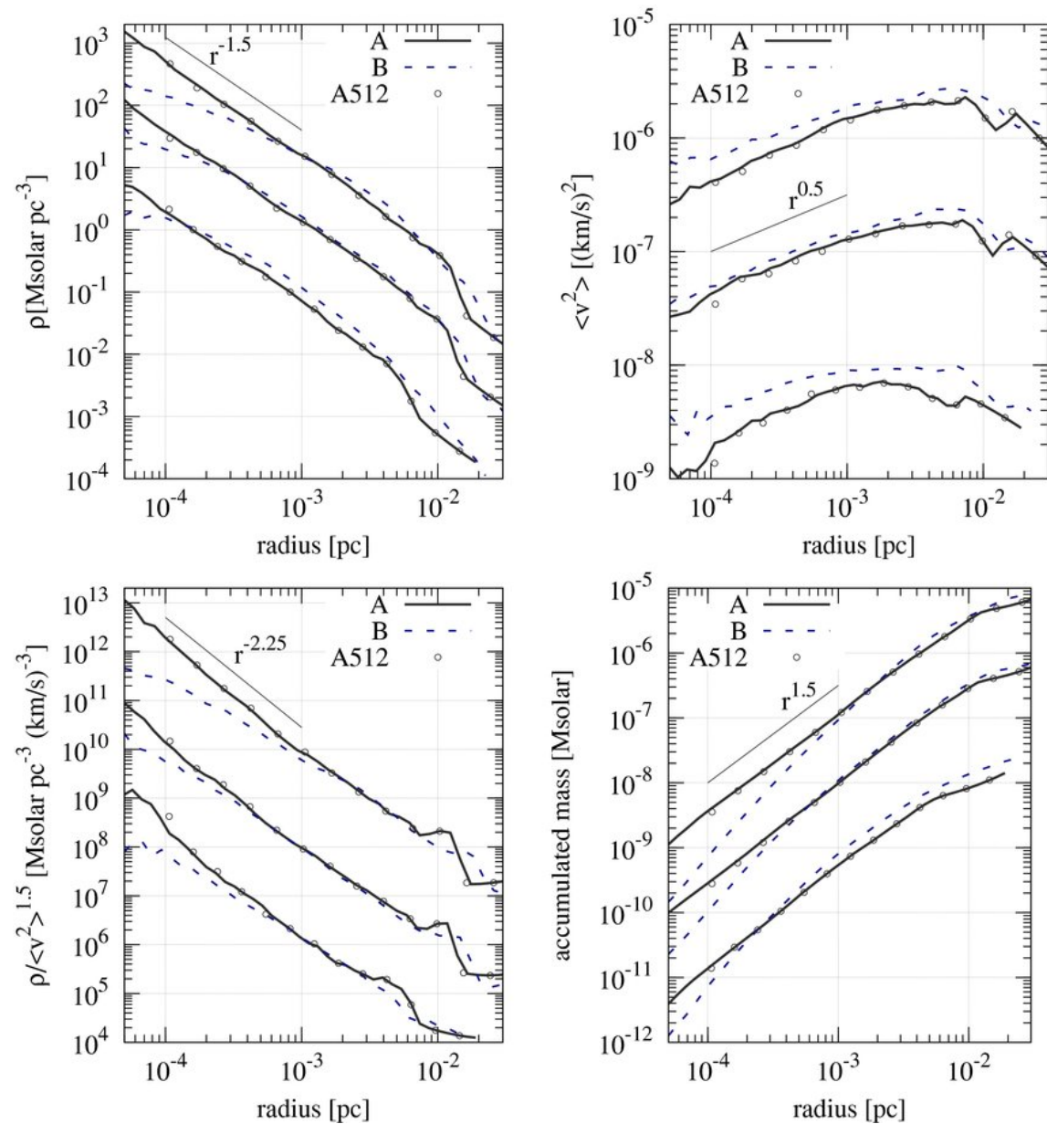
Figure 2. from Gamma-ray Signal from Earth-mass Dark Matter Microhalos ISHIYAMA, MAKINO, & EBISUZAKI 2010 ApJL 723 L195 doi:10.1088/2041-8205/723/2/L195 https://dx.doi.org/10.1088/2041-8205/723/2/L195 © 2010. The American Astronomical Society. All rights reserved.
