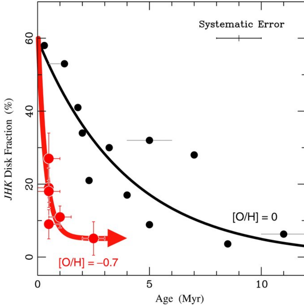
Figure 1. from Short Lifetime of Protoplanetary Disks in Low-metallicity Environments YASUI ET AL. 2010 ApJL 723 L113 doi:10.1088/2041-8205/723/1/L113 https://dx.doi.org/10.1088/2041-8205/723/1/L113 © 2010. The American Astronomical Society. All rights reserved.
