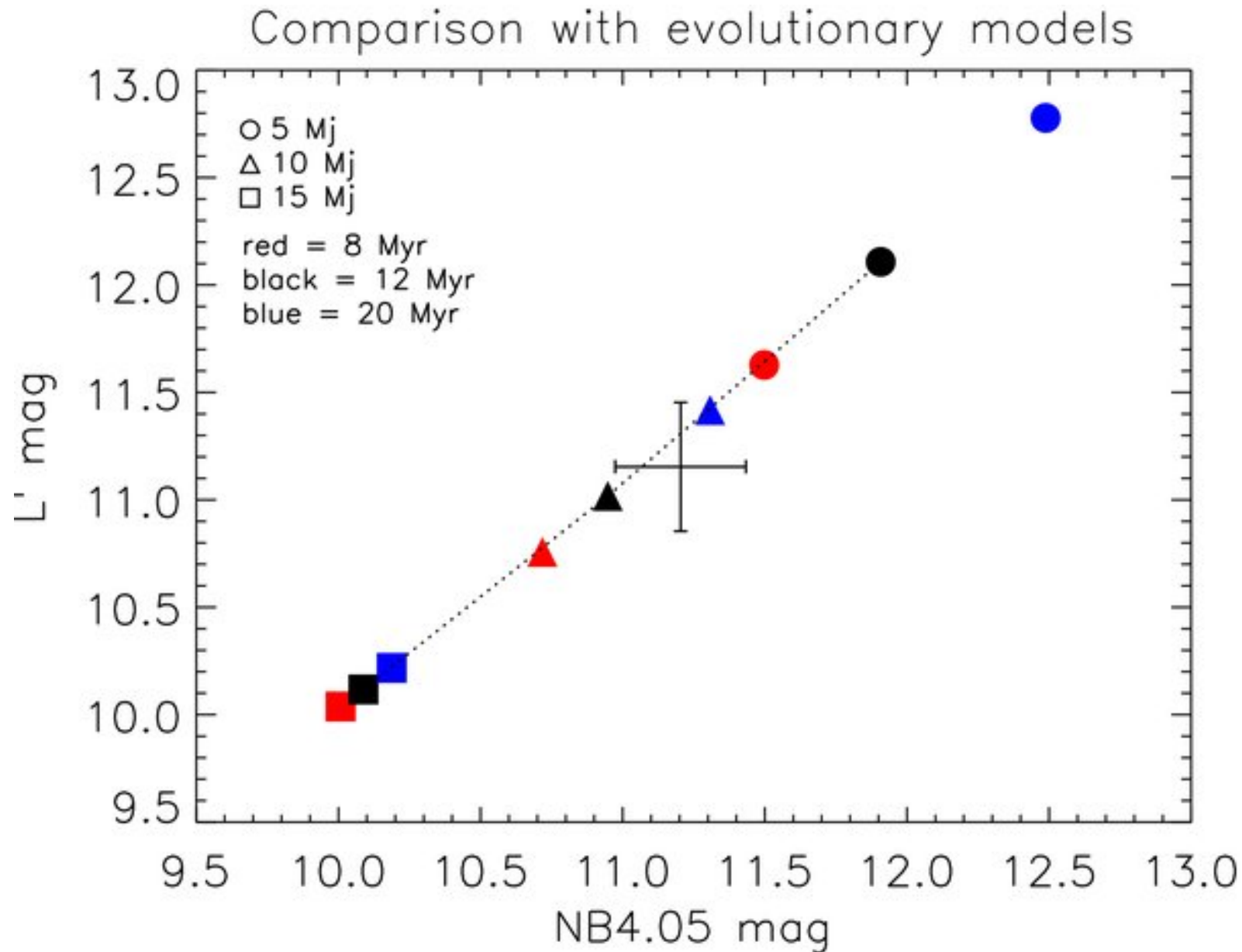
Figure 3. from First Results from Very Large Telescope NACO Apodizing Phase Plate: 4 m Images of The Exoplanet Pictoris b QUANZ ET AL. 2010 ApJL 722 L49 doi:10.1088/2041-8205/722/1/L49 https://dx.doi.org/10.1088/2041-8205/722/1/L49 © 2010. The American Astronomical Society. All rights reserved.
