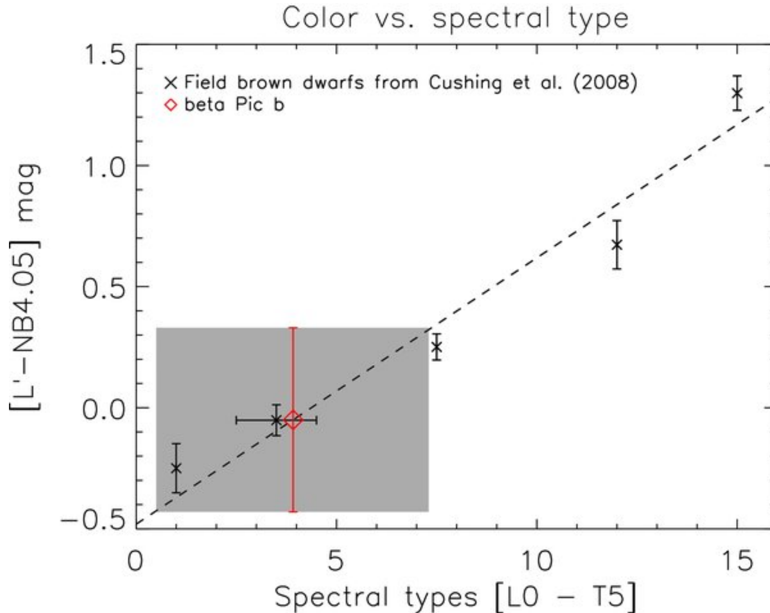
Figure 2. from First Results from Very Large Telescope NACO Apodizing Phase Plate: 4 m Images of The Exoplanet Pictoris b QUANZ ET AL. 2010 ApJL 722 L49 doi:10.1088/2041-8205/722/1/L49 https://dx.doi.org/10.1088/2041-8205/722/1/L49 © 2010. The American Astronomical Society. All rights reserved.
