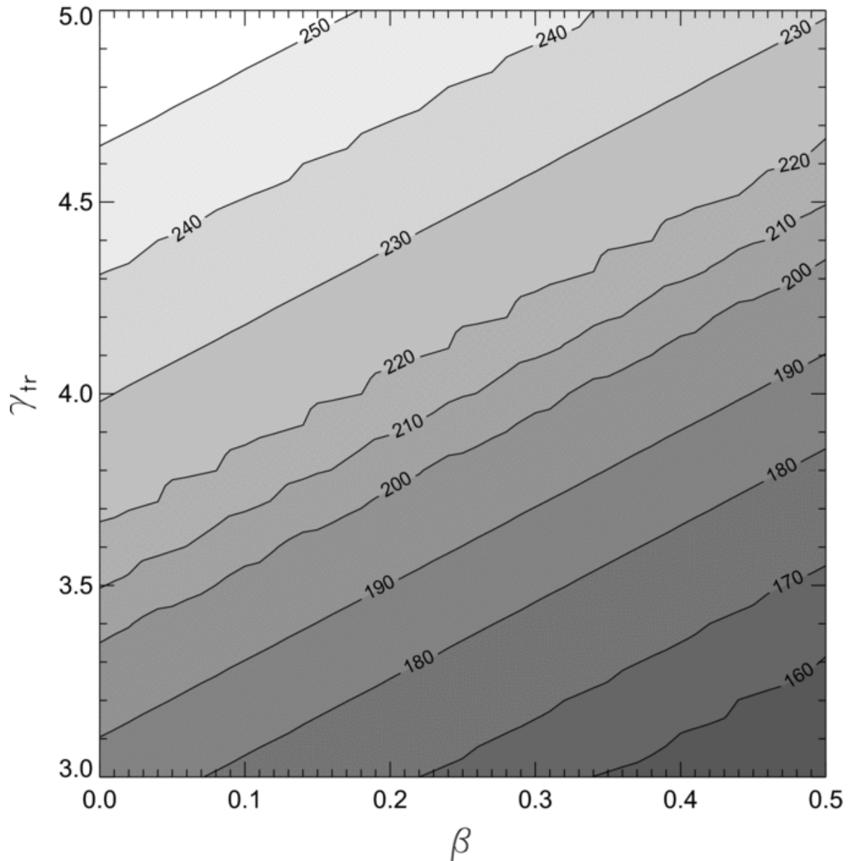
Figure 4. from The Mass Profile of the Galaxy to 80 kpc GNEDIN ET AL. 2010 ApJL 720 L108 doi:10.1088/2041-8205/720/1/L108 https://dx.doi.org/10.1088/2041-8205/720/1/L108 © 2010. The American Astronomical Society. All rights reserved.
