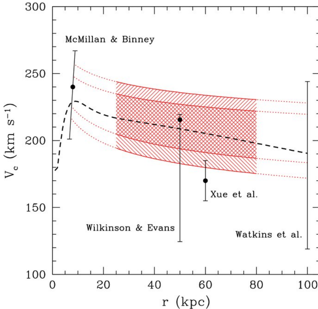
Figure 3. from The Mass Profile of the Galaxy to 80 kpc GNEDIN ET AL. 2010 ApJL 720 L108 doi:10.1088/2041-8205/720/1/L108 https://dx.doi.org/10.1088/2041-8205/720/1/L108 © 2010. The American Astronomical Society. All rights reserved.
