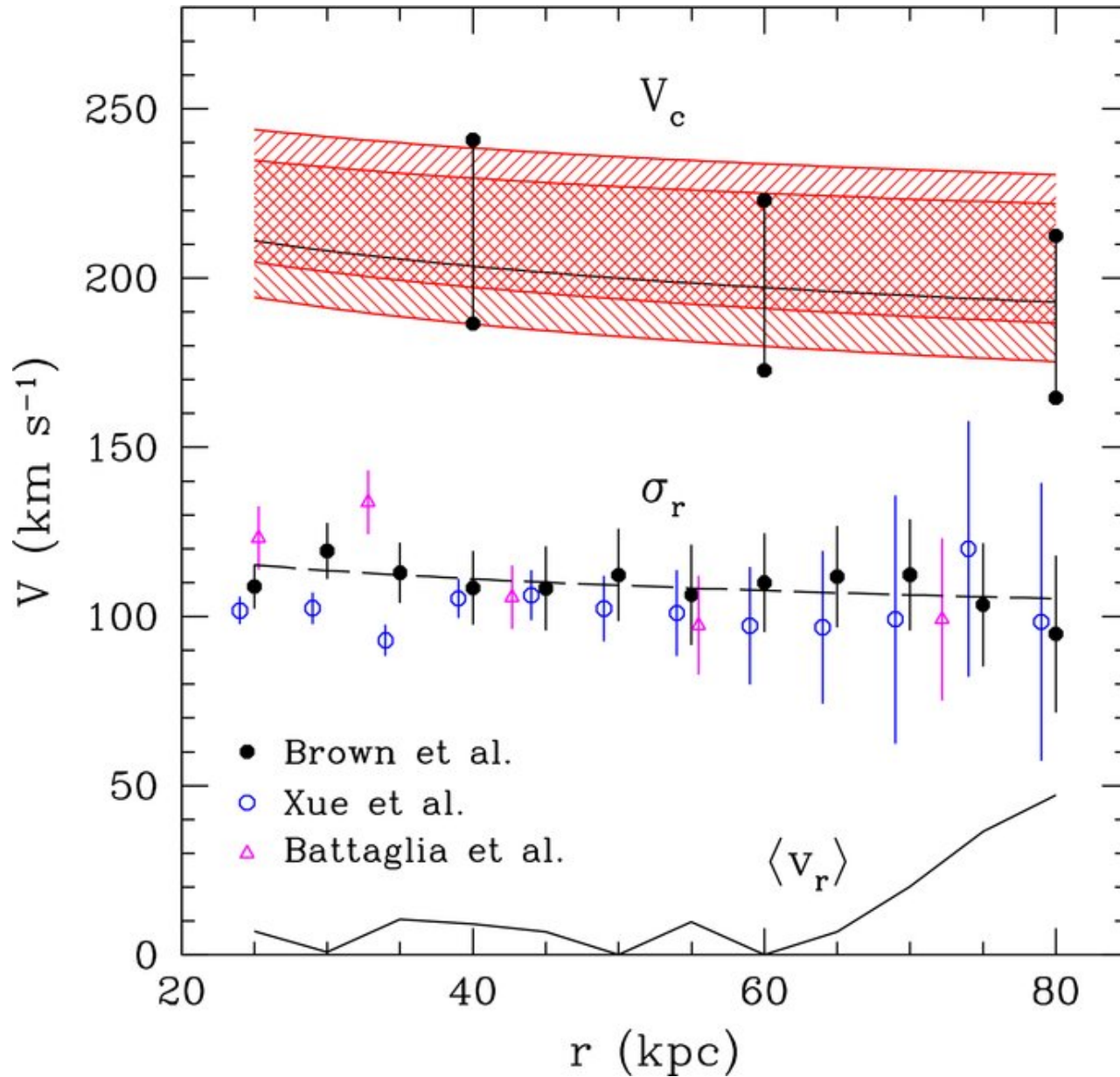
Figure 2. from The Mass Profile of the Galaxy to 80 kpc GNEDIN ET AL. 2010 ApJL 720 L108 doi:10.1088/2041-8205/720/1/L108 https://dx.doi.org/10.1088/2041-8205/720/1/L108 © 2010. The American Astronomical Society. All rights reserved.
