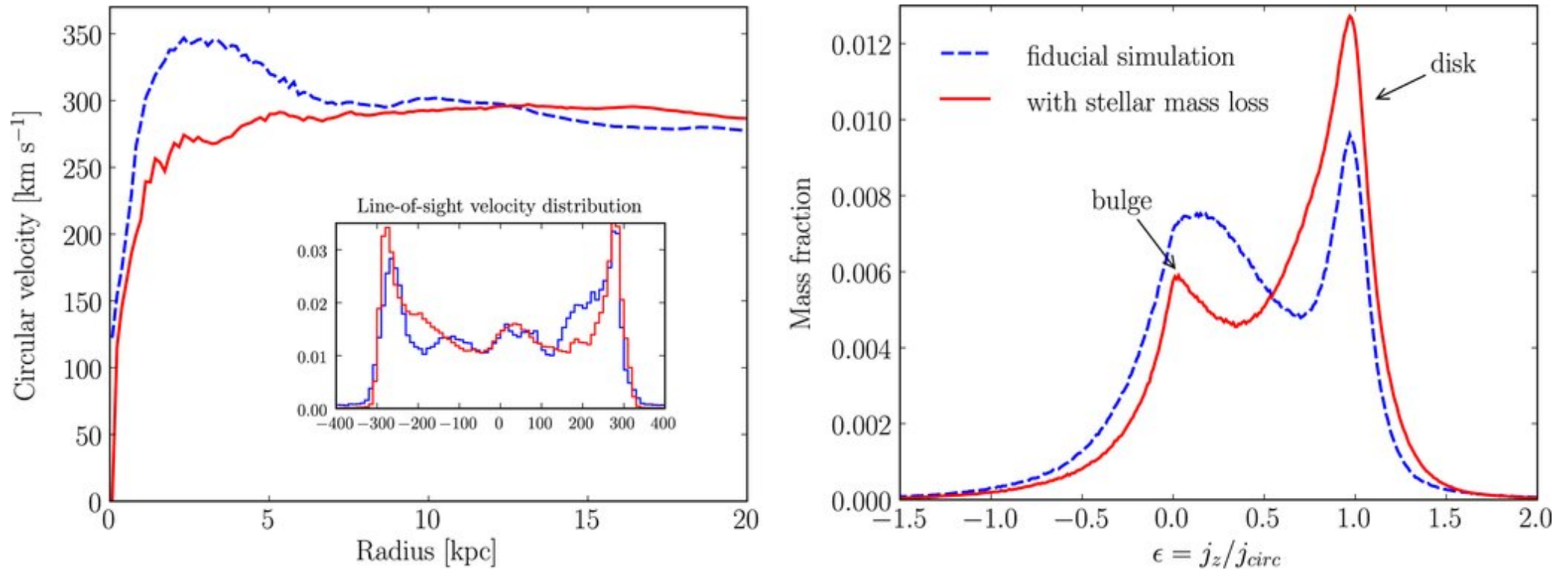
Figure 4. from Formation of Late-type Spiral Galaxies: Gas Return from Stellar Populations Regulates Disk Destruction and Bulge Growth MARTIG & BOURNAUD 2010 ApJL 714 L275 doi:10.1088/2041-8205/714/2/L275 https://dx.doi.org/10.1088/2041-8205/714/2/L275 © 2010. The American Astronomical Society. All rights reserved.
